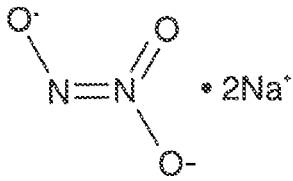
Angeli's salt
