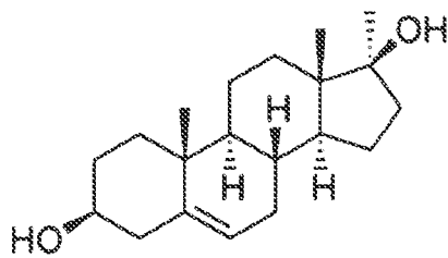
Methandriol
