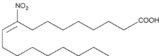
9-Nitrooleate
