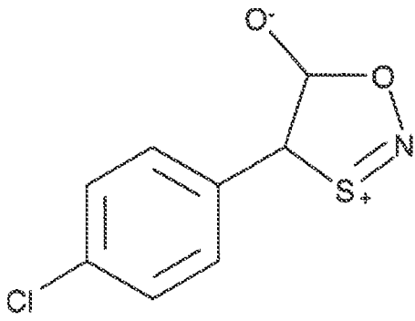
4-(p-chlorophenyl)-1,3,2-Oxathiazolylium-5-olate
