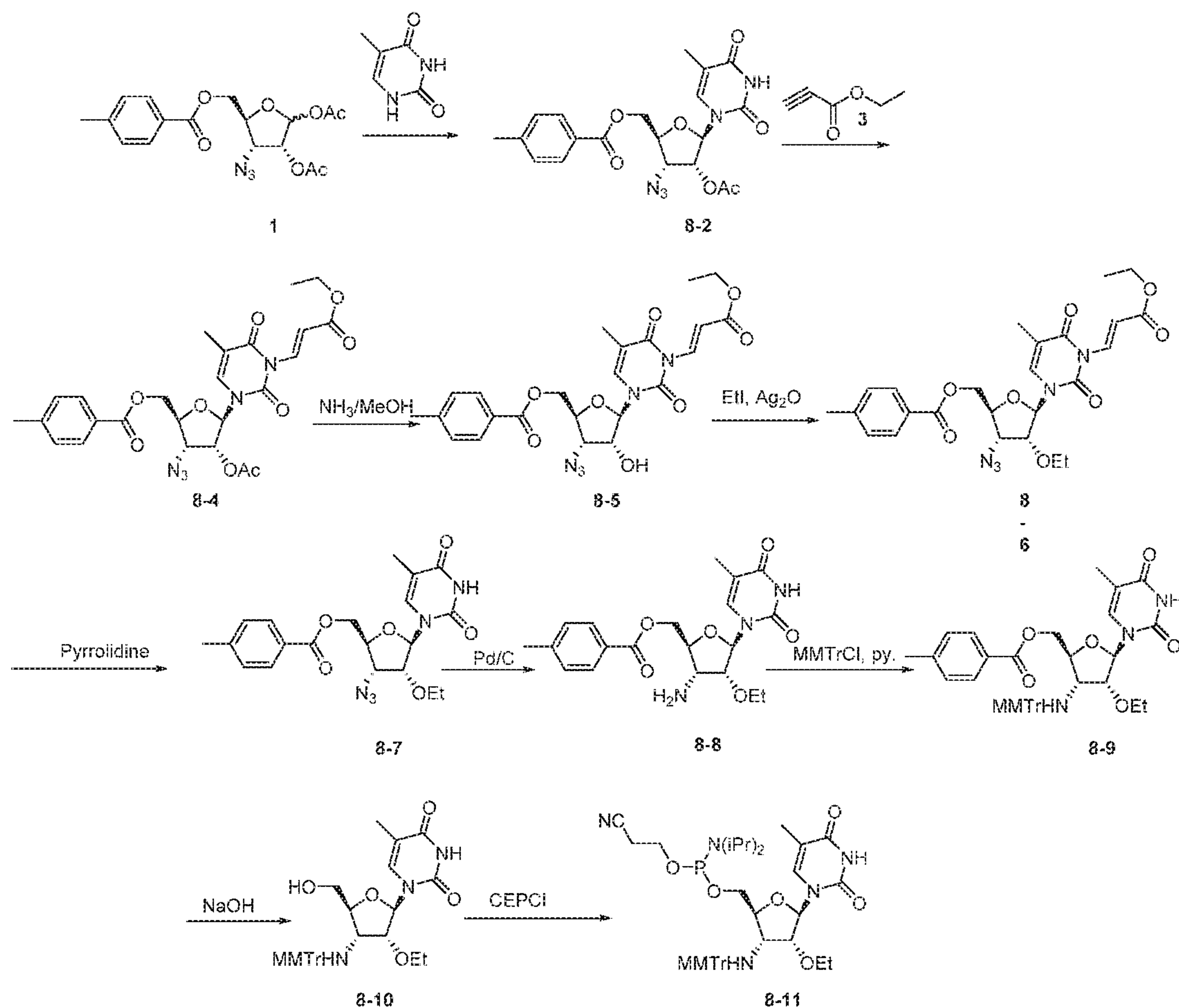
Scheme 5
