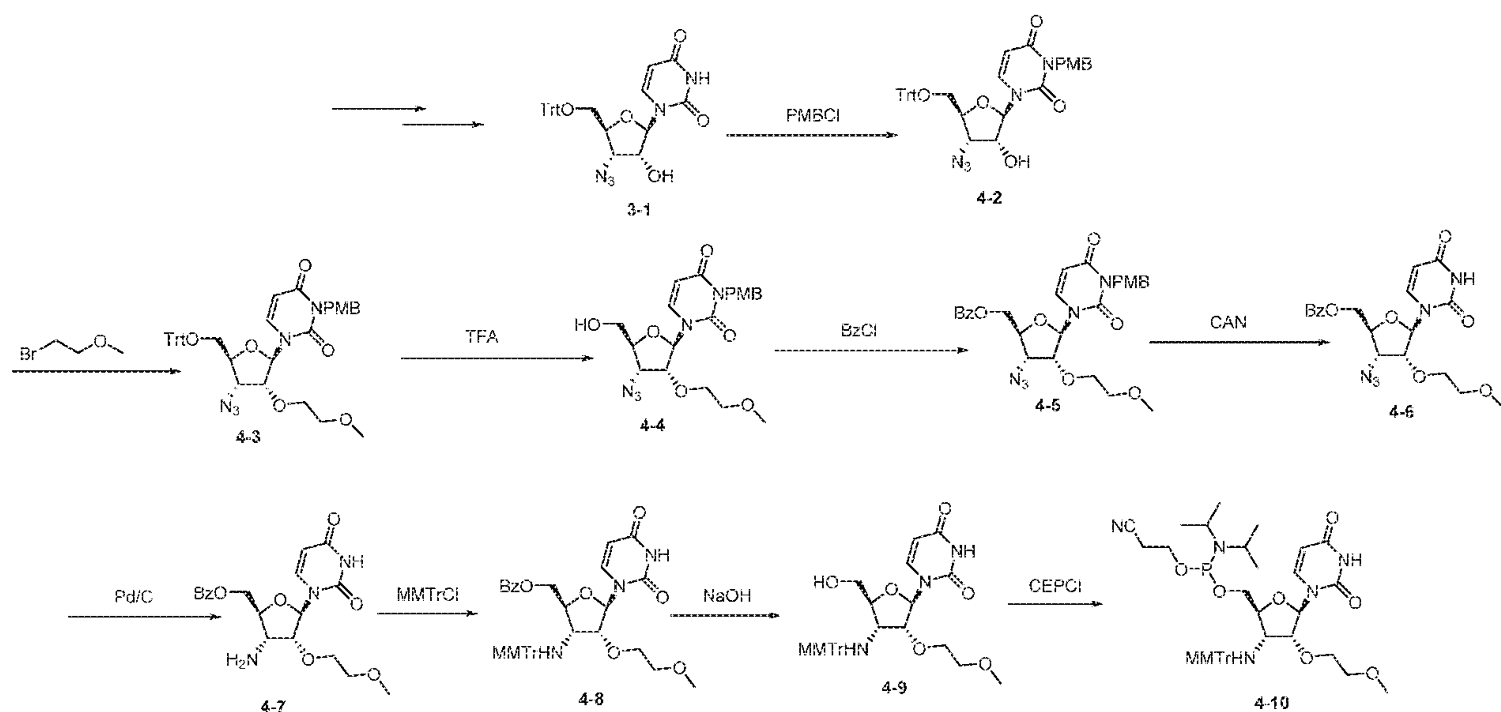
Scheme 2
