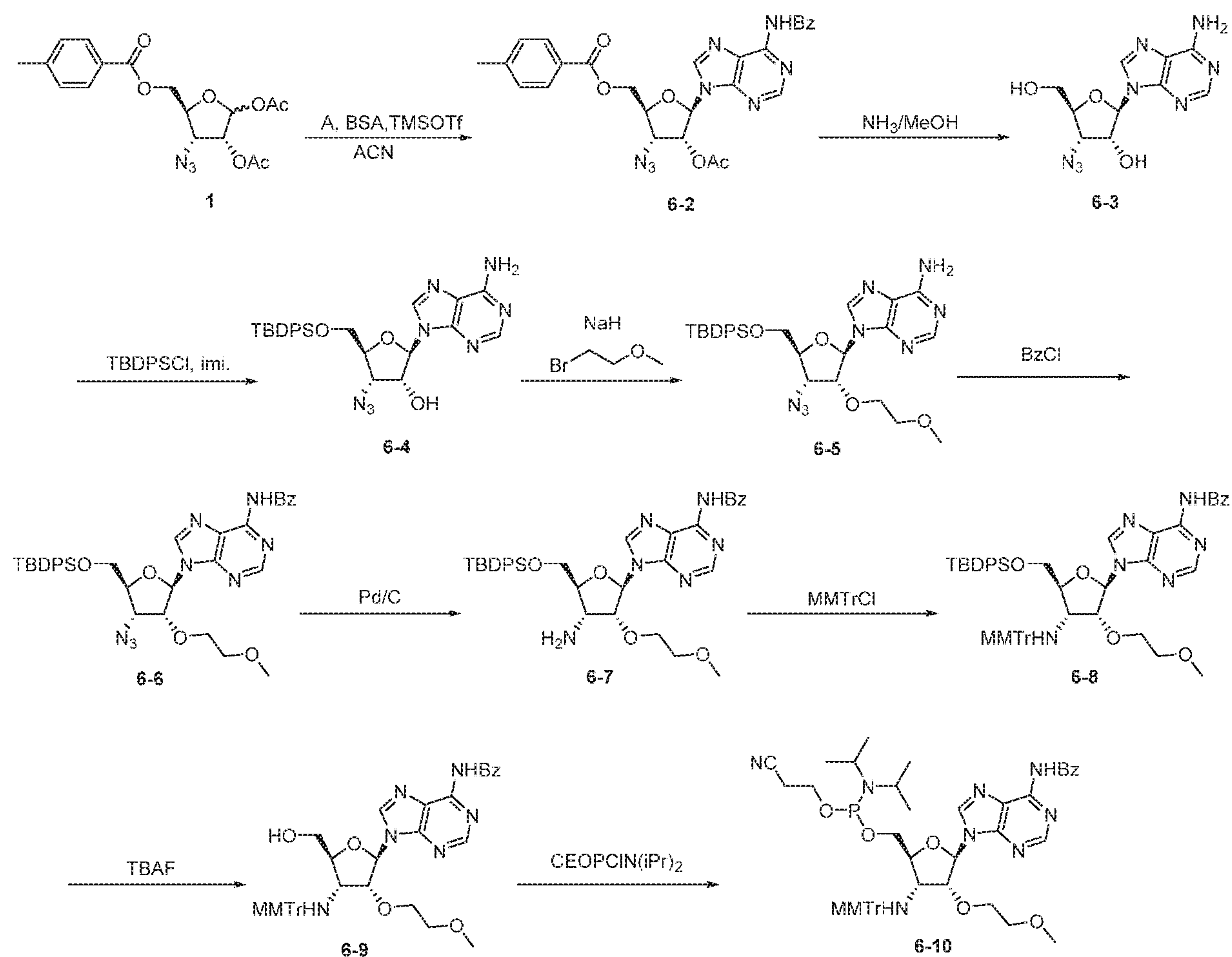
Scheme 4
