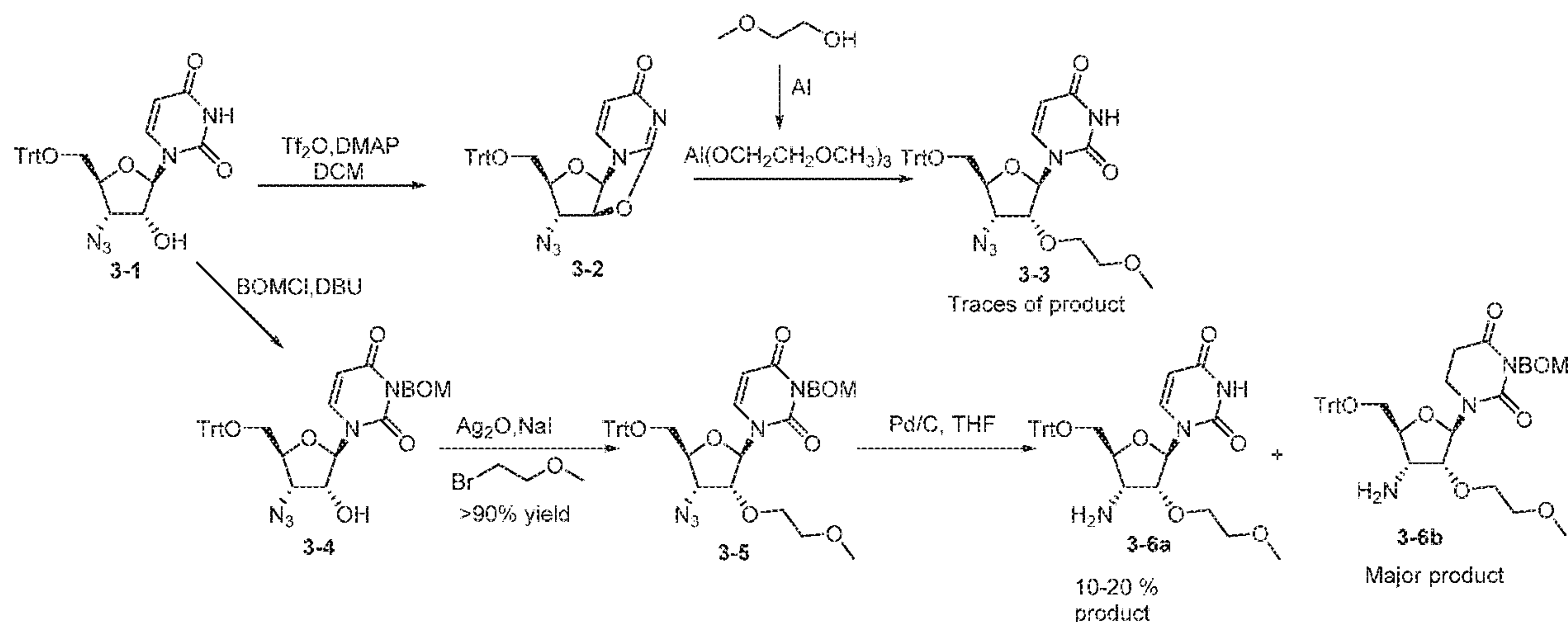
Scheme 1
