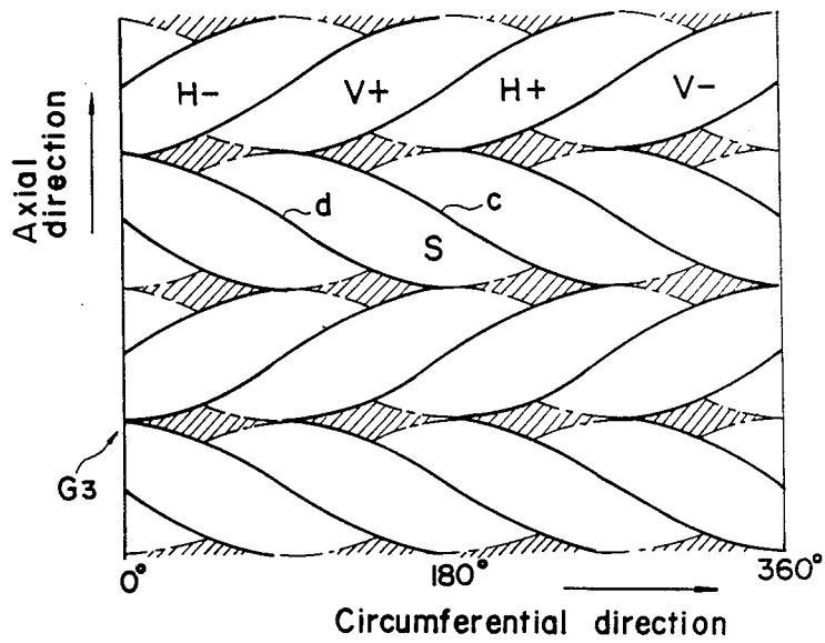
FIG. 6 (PRIOR ART)
