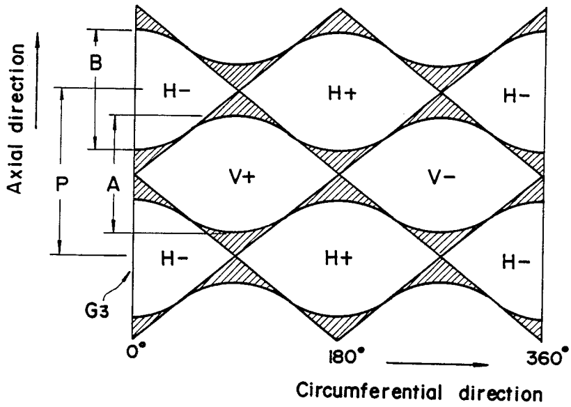
FIG. 5 (PRIOR ART)
