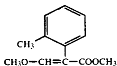
Methyl 3-methoxy-2-(2-methylphenyl)-acrylate (disclosed in EP 178,816)
