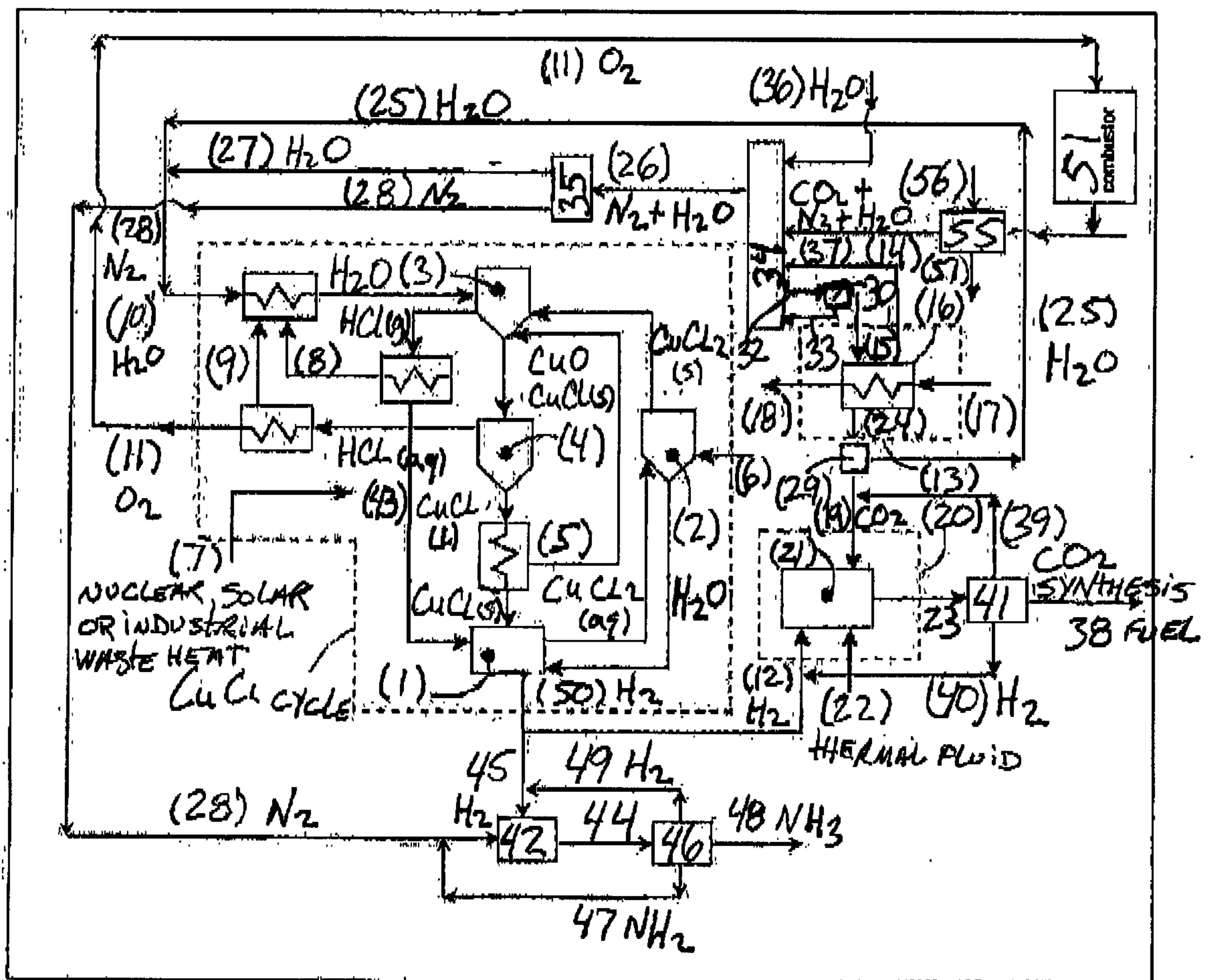
Figure 1: Schematic of the Cu-Cl cycle with \text{CO}_2 capture and hydrogenation (drying and hydrolysis processes of \text{CuCl}_2 and absorption of \text{CO}_2 are shown in separate apparatus)
