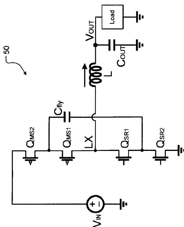
FIG. 1C Prior Art
