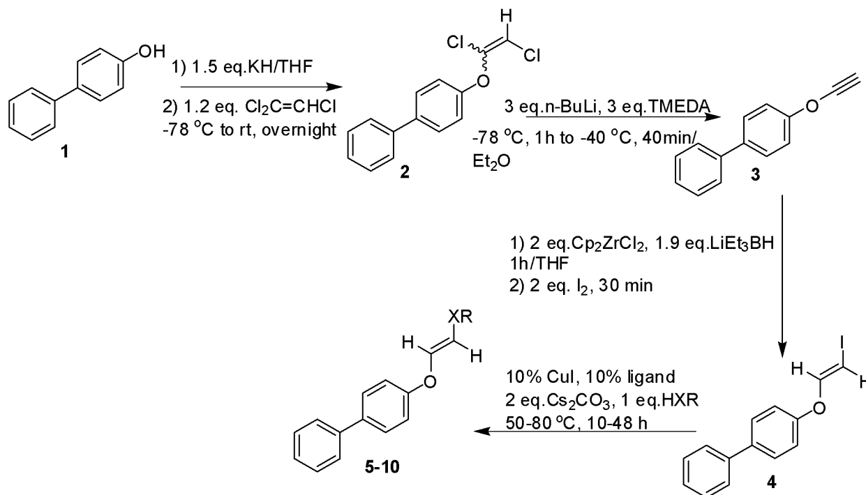
Scheme 3. Synthetic route for vinyl diether and its analogues
