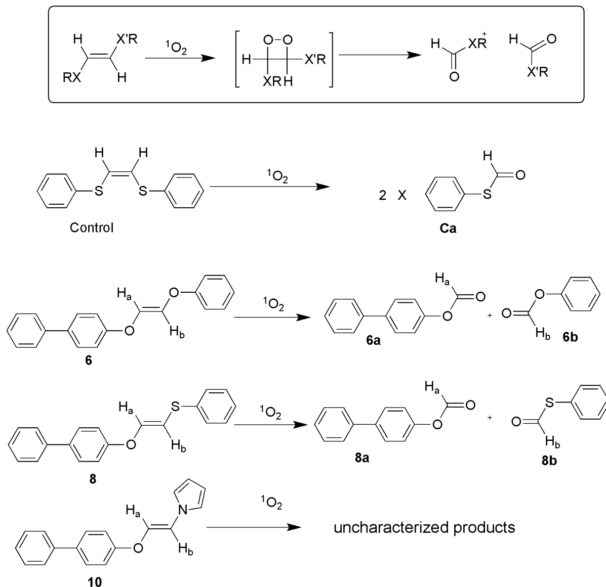
Scheme 4. Possible [2+2] addition reaction of electron-rich olefins with singlet oxygen and expected products of control, 6 , 8 , and 10 .
