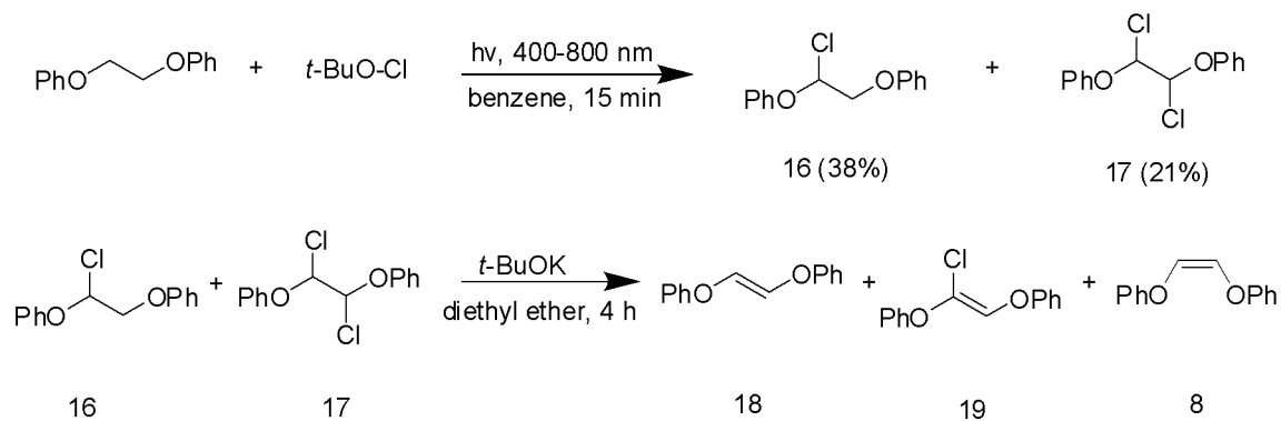
SCHEME 2. Synthetic scheme for the preparation of 8
