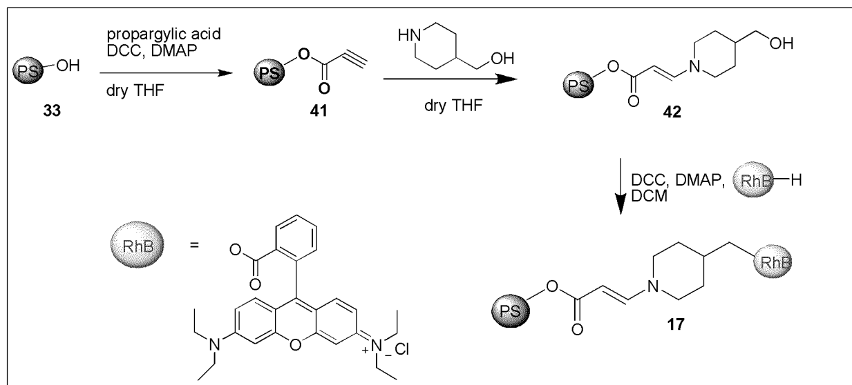
Scheme 5. Synthetic routes of the substrates
