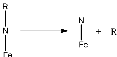
Reaction 3
