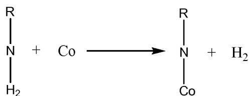
Reaction 1
