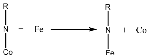
Reaction 2
