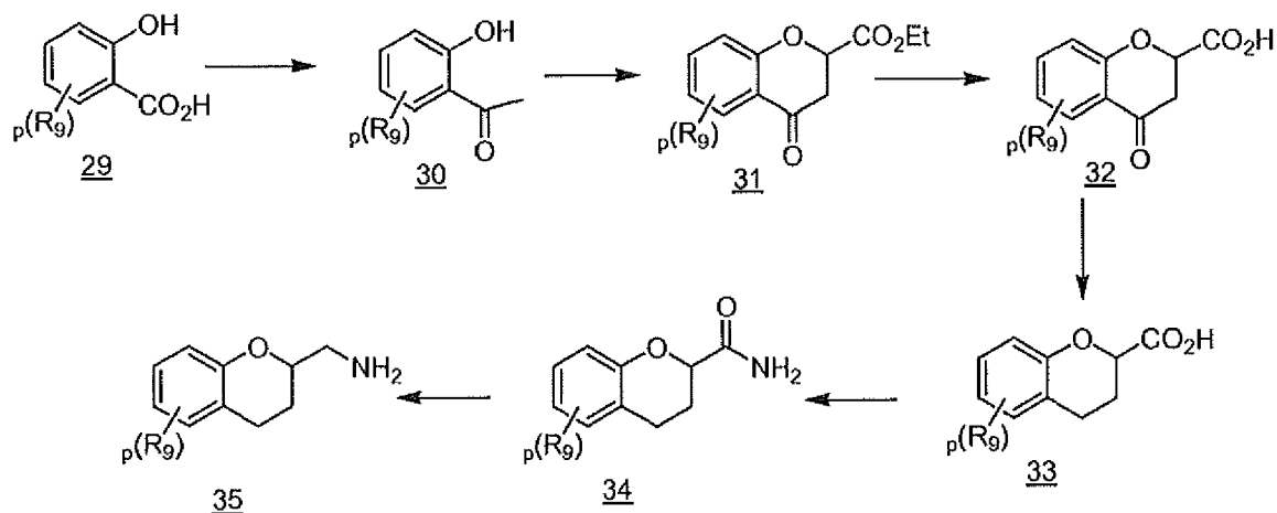
Scheme 9
