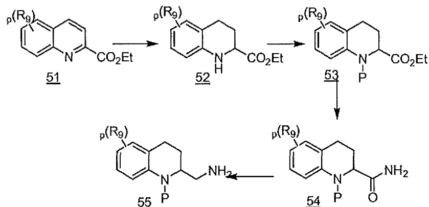
Scheme 13
