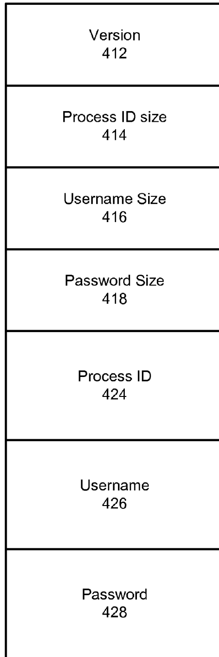
Logon Handle Request Structure 410
