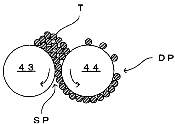
FIG. 4A : GREAT RESIDUAL QUANTITY OF TONER
