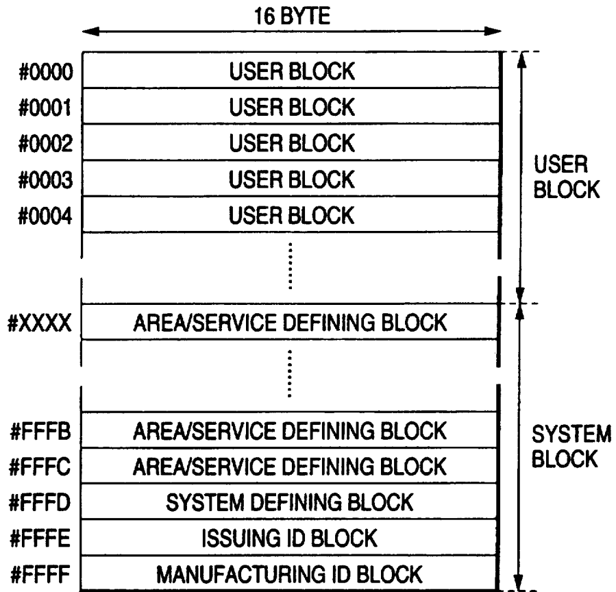
LOGICAL FORMAT OF EEPROM 66
