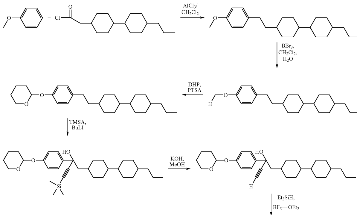
Scheme 7:
