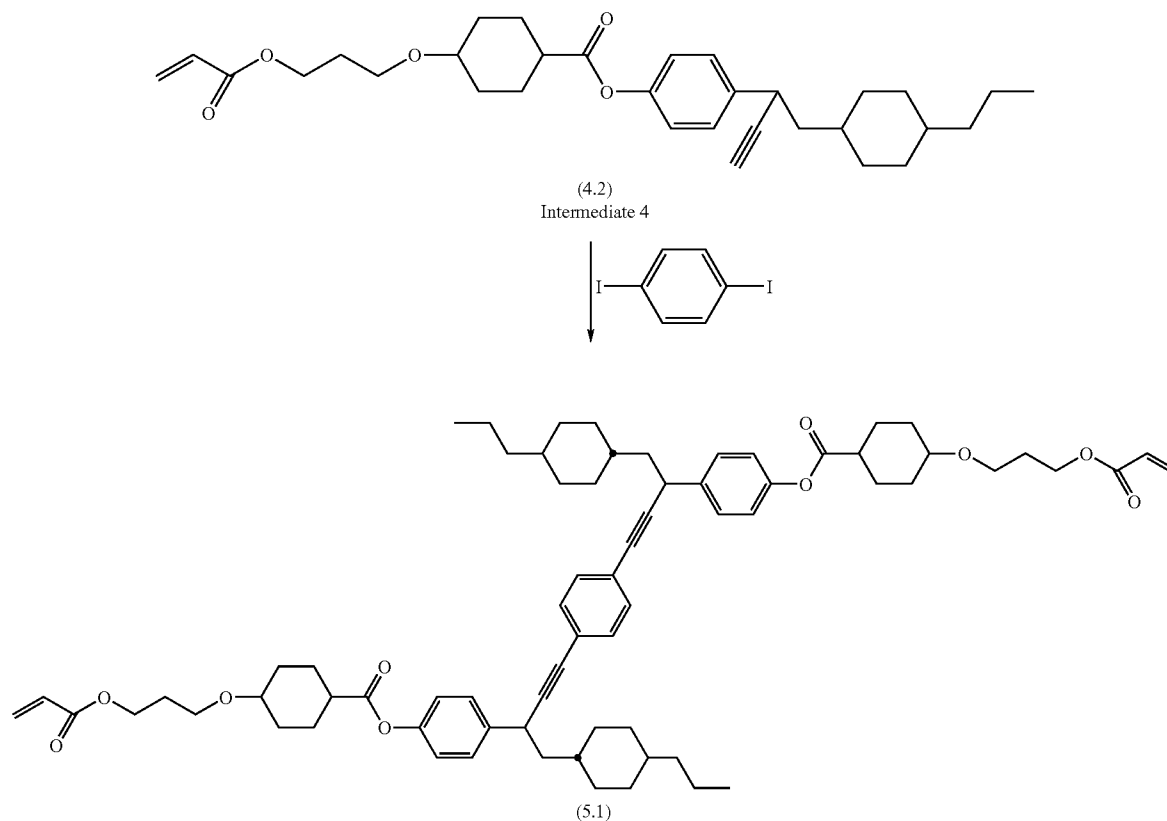
Scheme 5:
