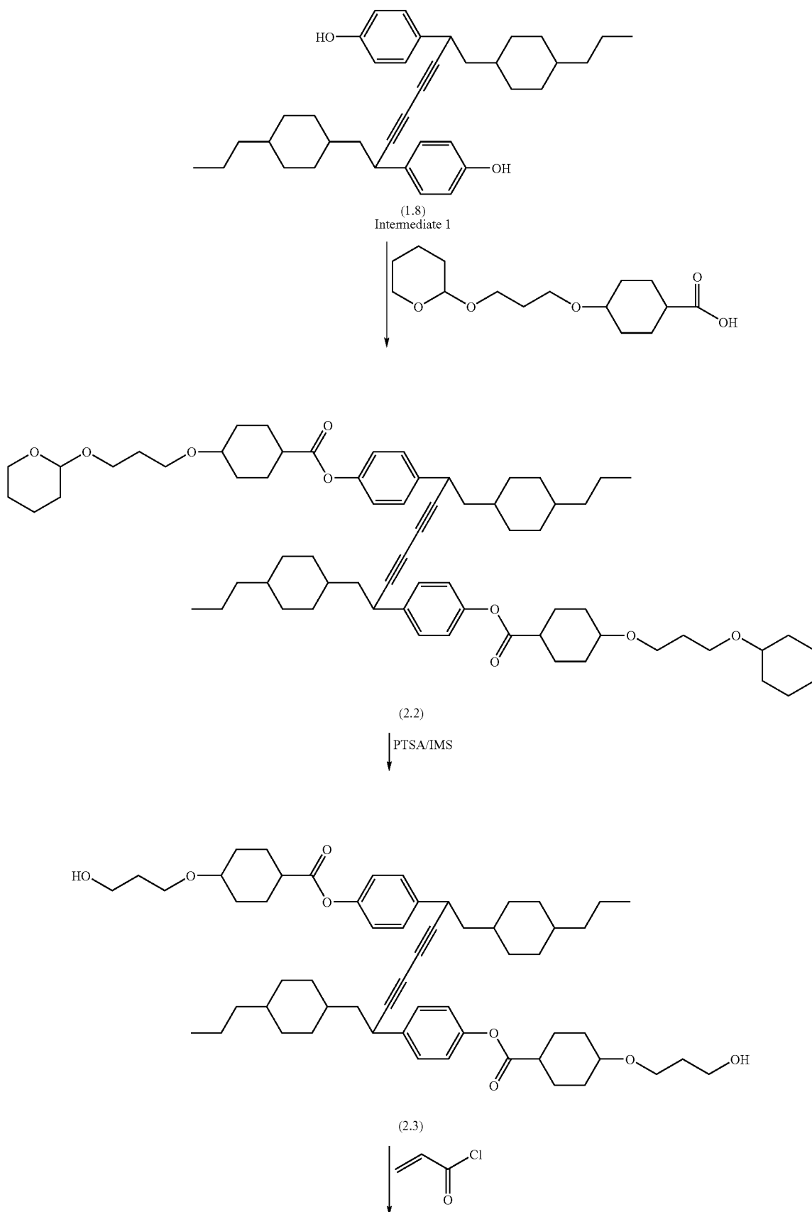
Scheme 2:
