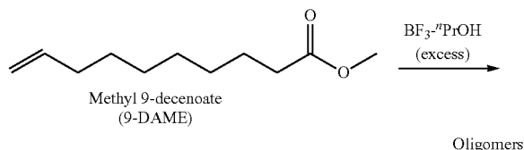
Scheme 1. BF 3 -mediated homo-oligomerization of methyl 9-decenoate (9-DAME).
