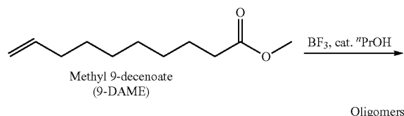
Scheme 1. \text{BF}_3 -mediated homo-oligomerization of methyl 9-decenoate.
