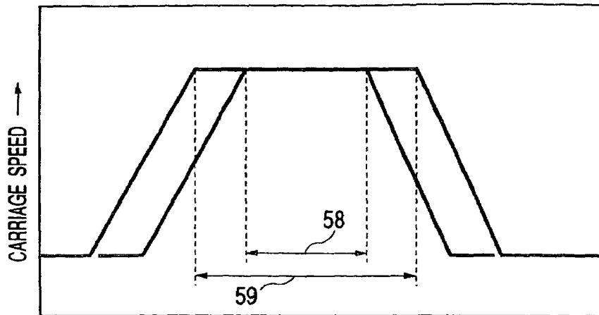
OPERATION RANGE OF CARRIAGE DURING STEP-PRINTING OPERATION
