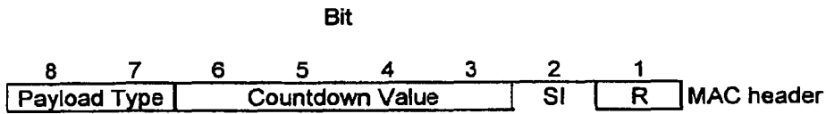
FIG. 3 PRIOR ART
