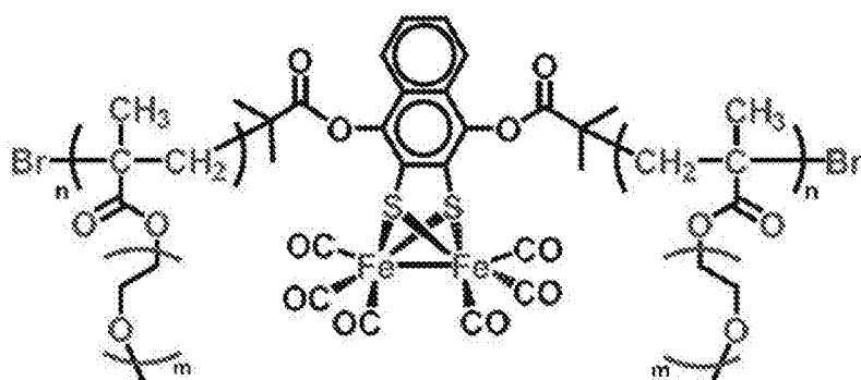
(PEGMA-g-[2Fe-2S]), and
