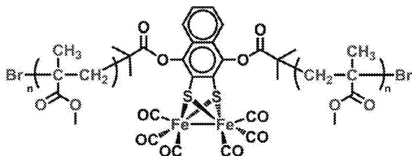
(PMMA-g-[2Fe-2S]),
