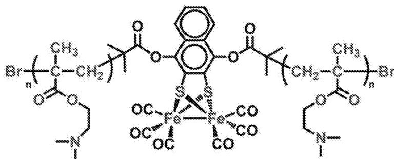
(PDMAEMA-g-[2Fe-2S]),
