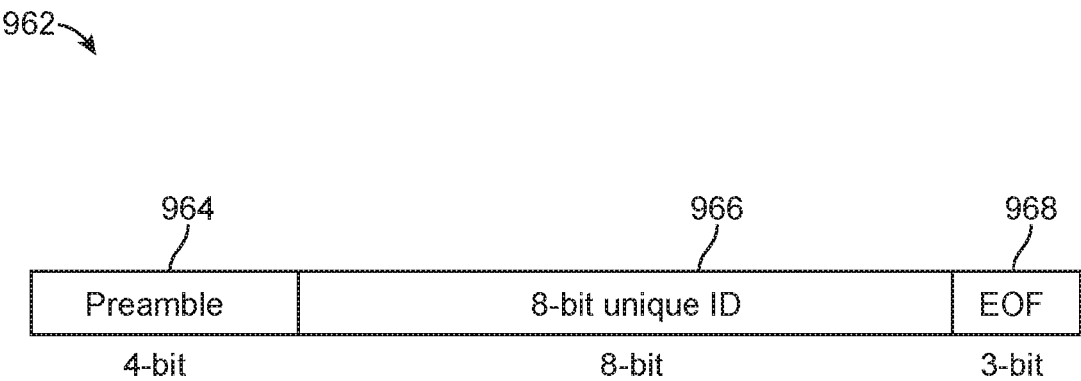
Packet structure
