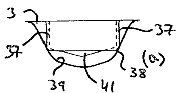
FIGURE 13 (PRIOR ART)
