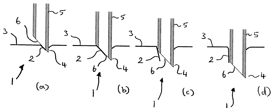
FIGURE 1 (PRIOR ART)
