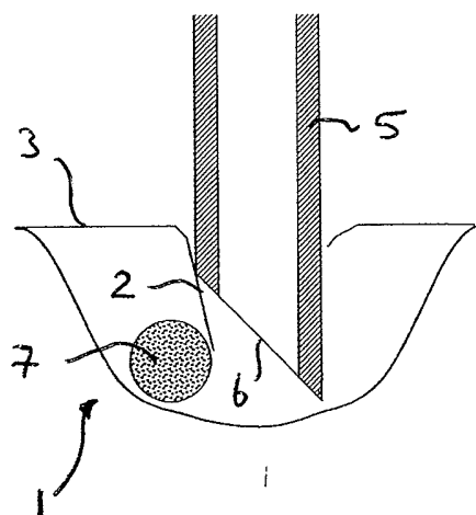
FIGURE 4 (PRIOR ART)
