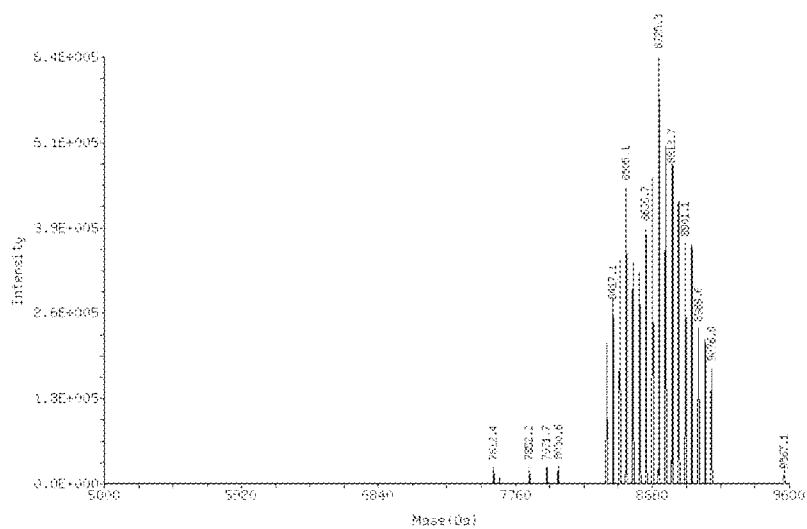
Fig. 18 ESI Mass Spectral analysis of 21-mer RNA with 3'-PEG-2000 attachment, purified RNA as shown in Fig. 17
