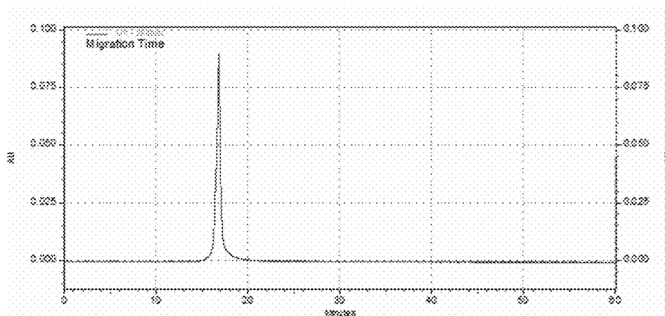
Fig. 13. 21- Mer RNA with 3'-Cholesterol-TEG linker Reverse direction (5'→3') synthesis and HPLC purification
