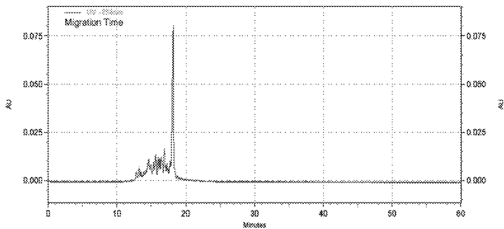
Fig.14 Electropherogram of the crude oligonucleotide, SEQ ID No. 3 made by reverse RNA synthesis
