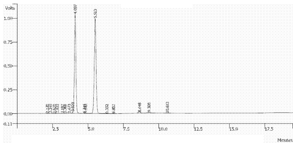
Fig.3. HPLC Chromatogram of the compound (16c)
