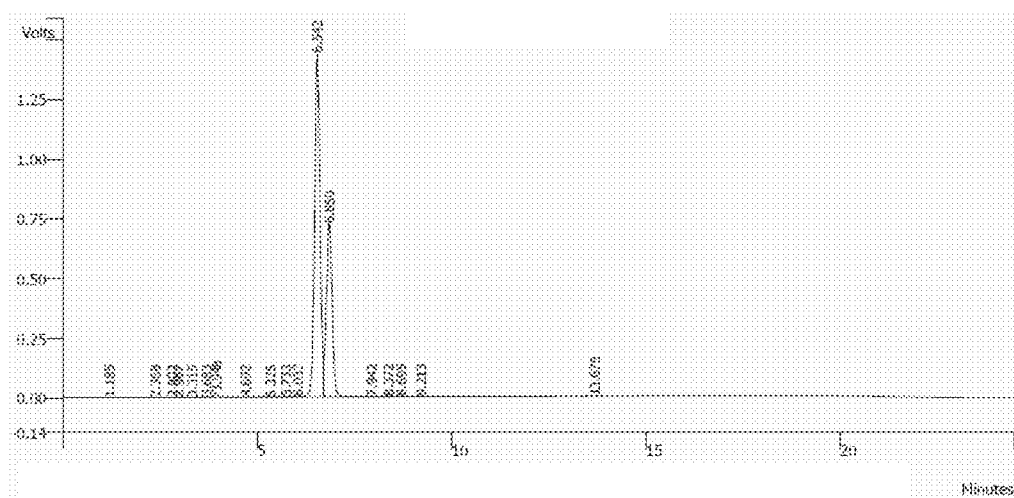
Fig.5. HPLC Chromatogram of the compound (16d)
