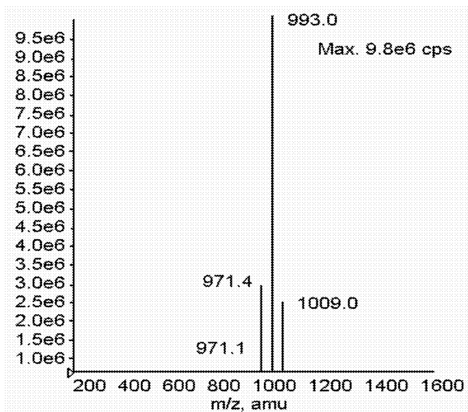
Fig.6b. Mass spectrum of the compound (16d)
