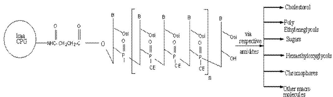
Fig.7. Diagrammatic Representation of 5'→3' RNA synthesis and application to 3'-modifications
