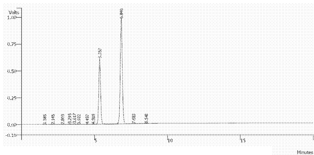
Fig.1. HPLC Chromatogram of the compound (16a)
