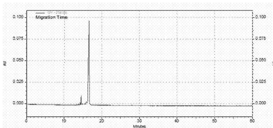
Fig.15 21-mer RNA synthesized by reverse direction ( 5' \rightarrow 3' ), followed by HEG (Hexa-ethyloxyglycol) attachment
