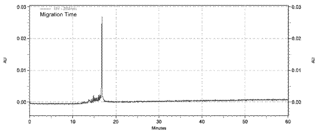
Fig.10 Electropherogram of the crude Oligonucleotide SEQ No.1 made by Reverse RNA synthesis
