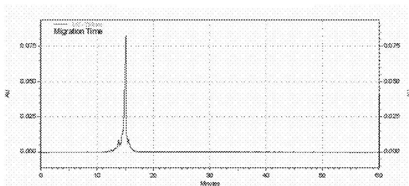
Fig. 9a. Electropherogram of the purified Oligonucleotide SEQ No.1 made by conventional method (3'-5'-direction)
