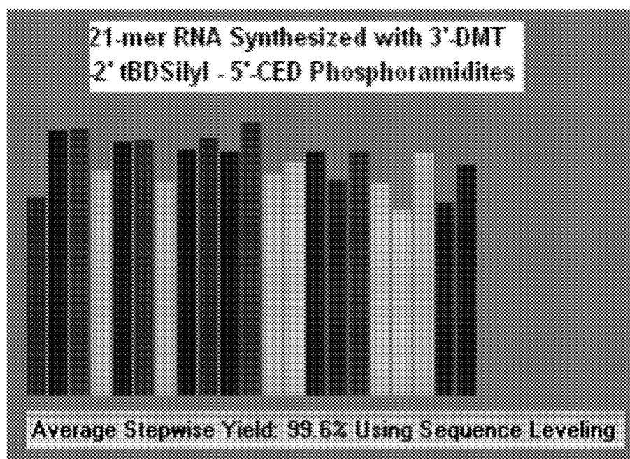
Fig. 8. Coupling Efficiency Trityl Histogram Notes (21 mer RNA Synthesis)
