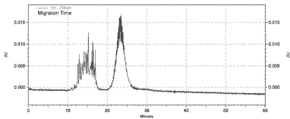
Fig. 16 Electropherogram of the crude oligonucleotide, SEQ ID No. 4 made by reverse RNA synthesis
