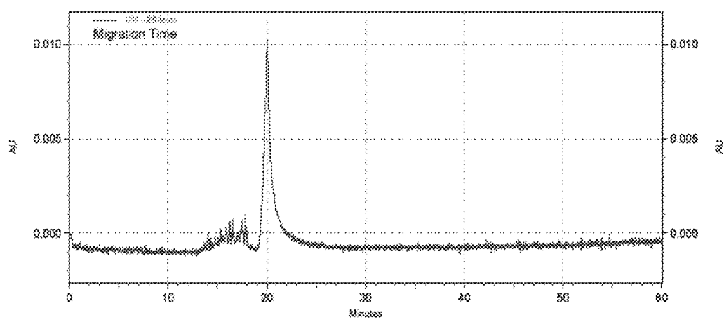
Fig. 12. Electropherogram of the crude oligonucleotide, SEQ ID No. 2 made by reverse RNA synthesis
