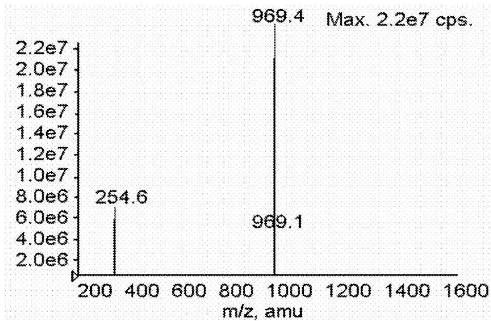
Fig.6a. Mass spectrum of the compound (16d)
