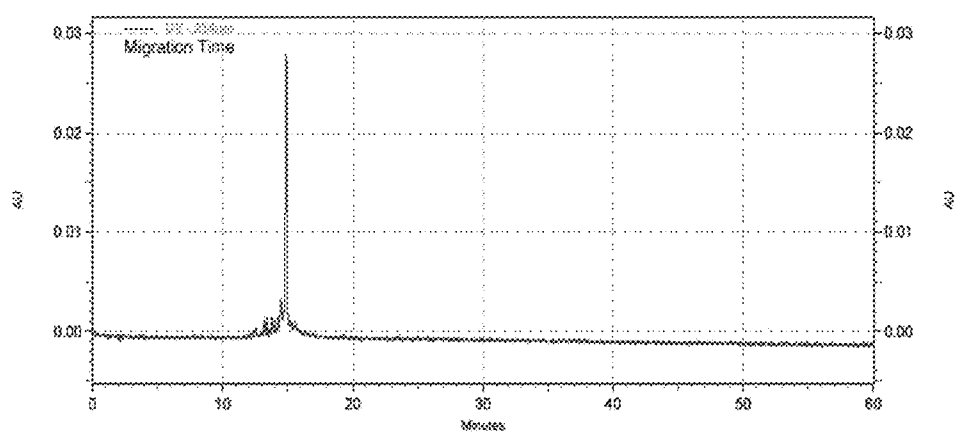
Fig. 9. Electropherogram of the crude Oligonucleotide SEQ No.1 made by conventional method (3'-5'-direction)
