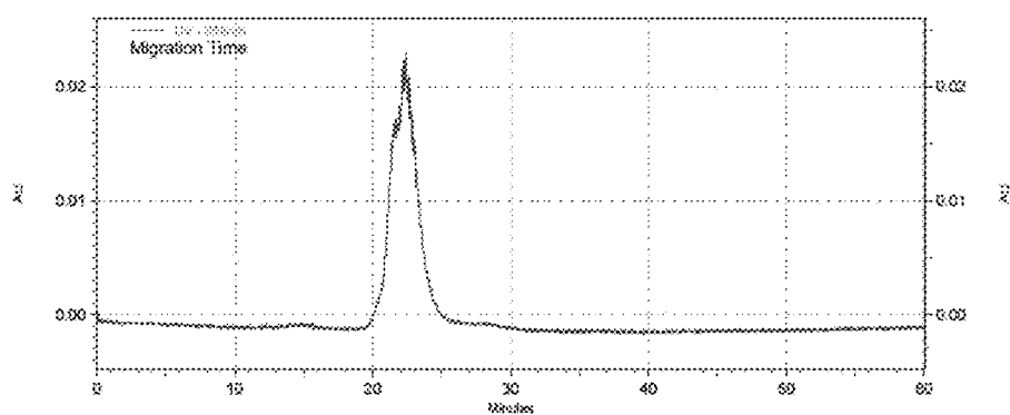
Fig. 17 Electropherogram of the crude oligonucleotide, SEQ ID No. 4 made by reverse RNA synthesis and purified by reverse-phase HPLC
