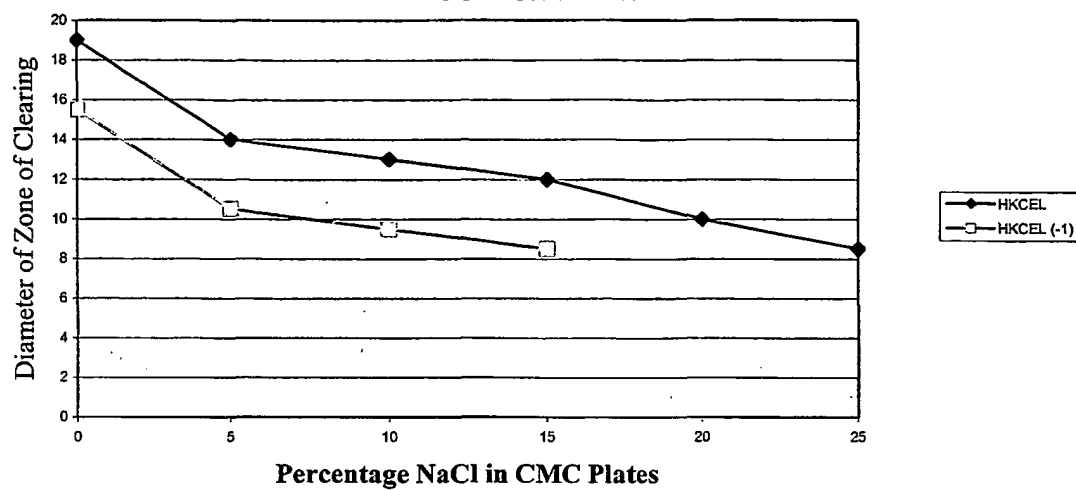
Figure 4 . Enzyme Activity with Increasing NaCl Concentration
