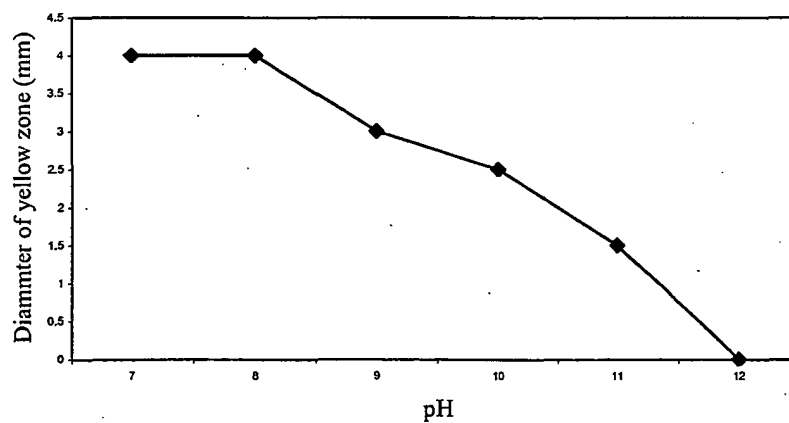
Figure 5. Influence of pH on mHKcel Cellulase Activity
