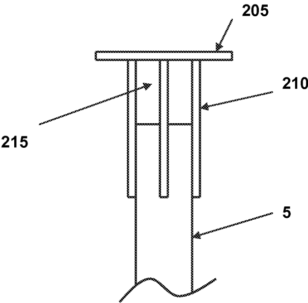
Elevation View
