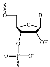
RNA
