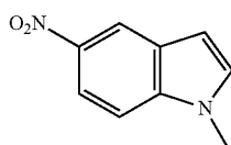
5-Nitroindole
