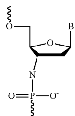
3'-Phosphoramidate
