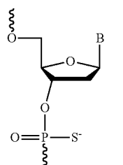
Phosphorothioate
