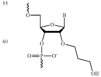
2'-(3-hydroxy)propyl
