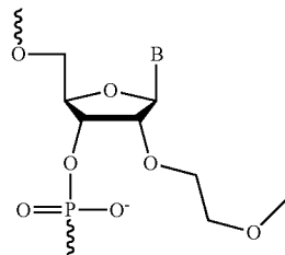
2'-MOE
