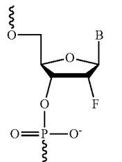
2'-Fluoro
