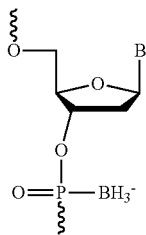
Boranophosphates
