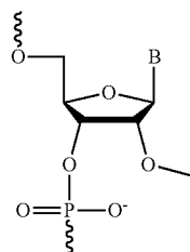
2'-O-Methyl
