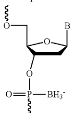
Boranophosphates
