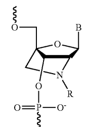
Amino-LNA
