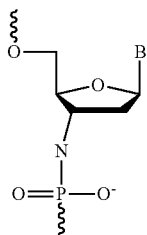
3'-Phosphoramidate
