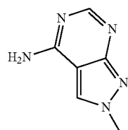
N 8 -8aza-7deazaadenine
