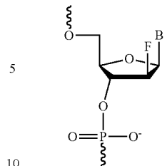
2'-F-ANA
