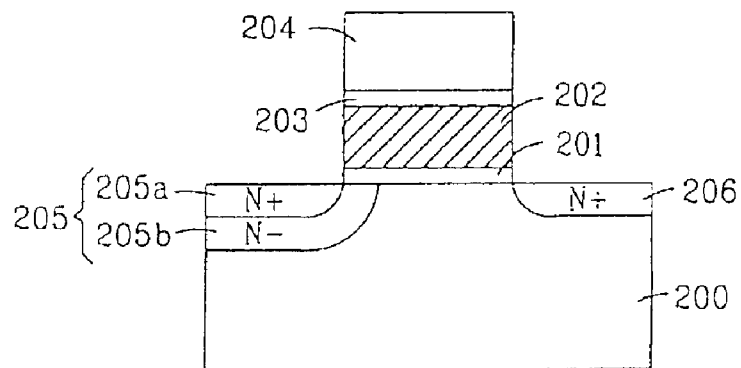
FIG. 2 BACKGROUND ART
