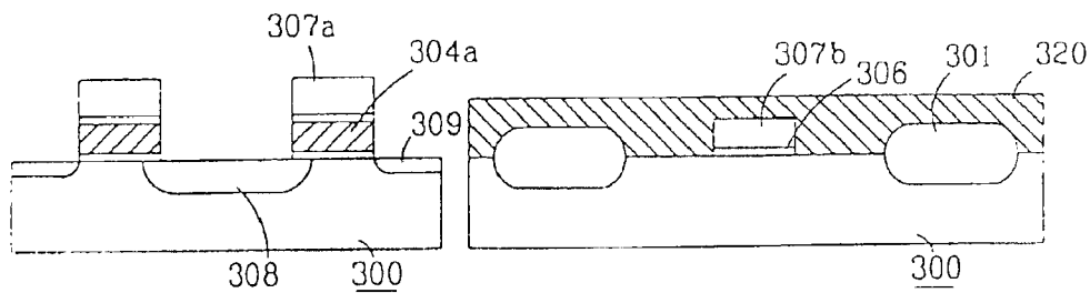
FIG. 3C BACKGROUND ART
