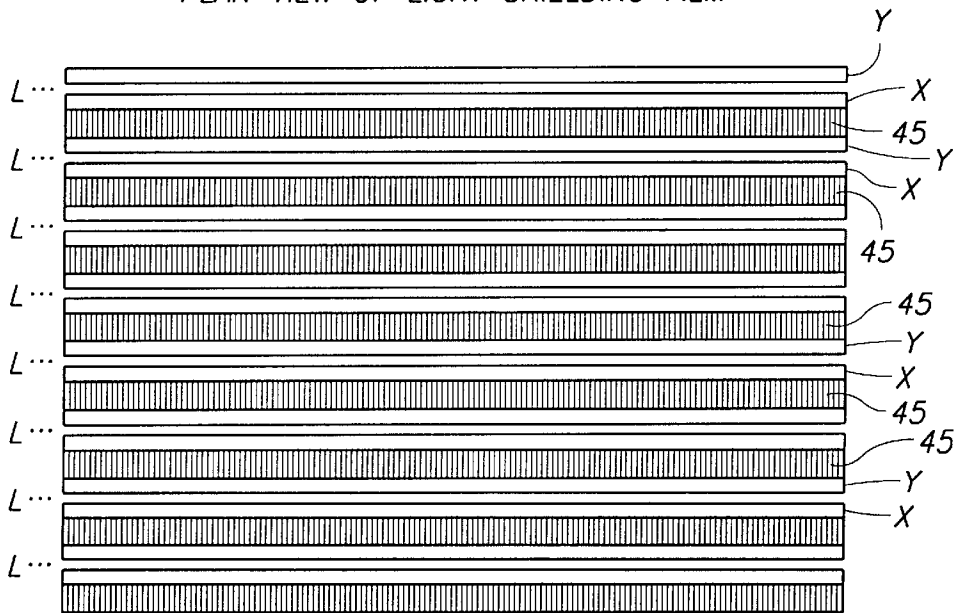
PLAN VIEW OF LIGHT SHIELDING FILM
