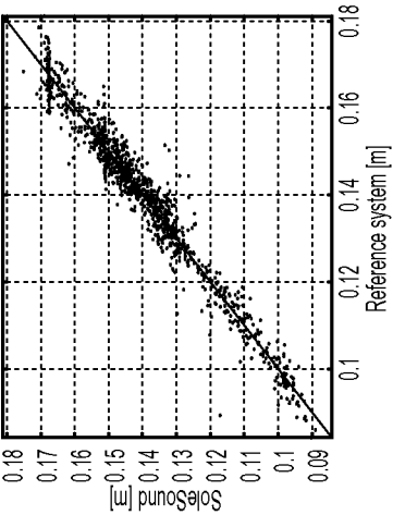
Foot-Ground clearance
