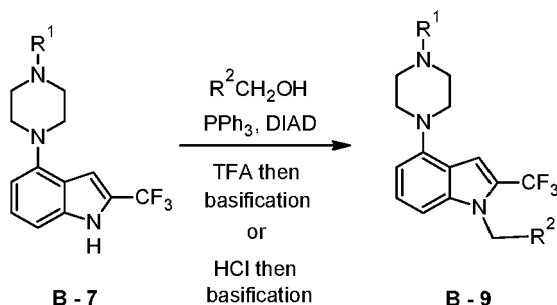
Reaction Scheme 6.
