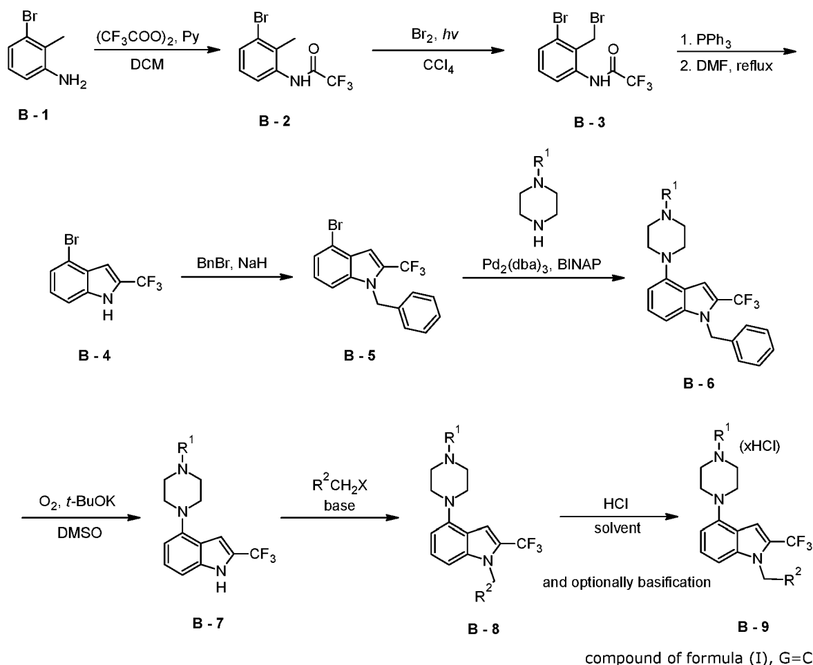
Reaction Scheme 5.
