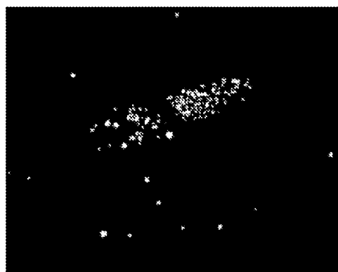
alpha-L-oxy-LNA; 2774
