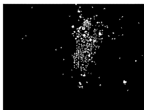
beta-D-thio-LNA; 2746
