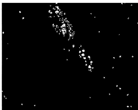
beta-D-oxy-LNA; 2740
