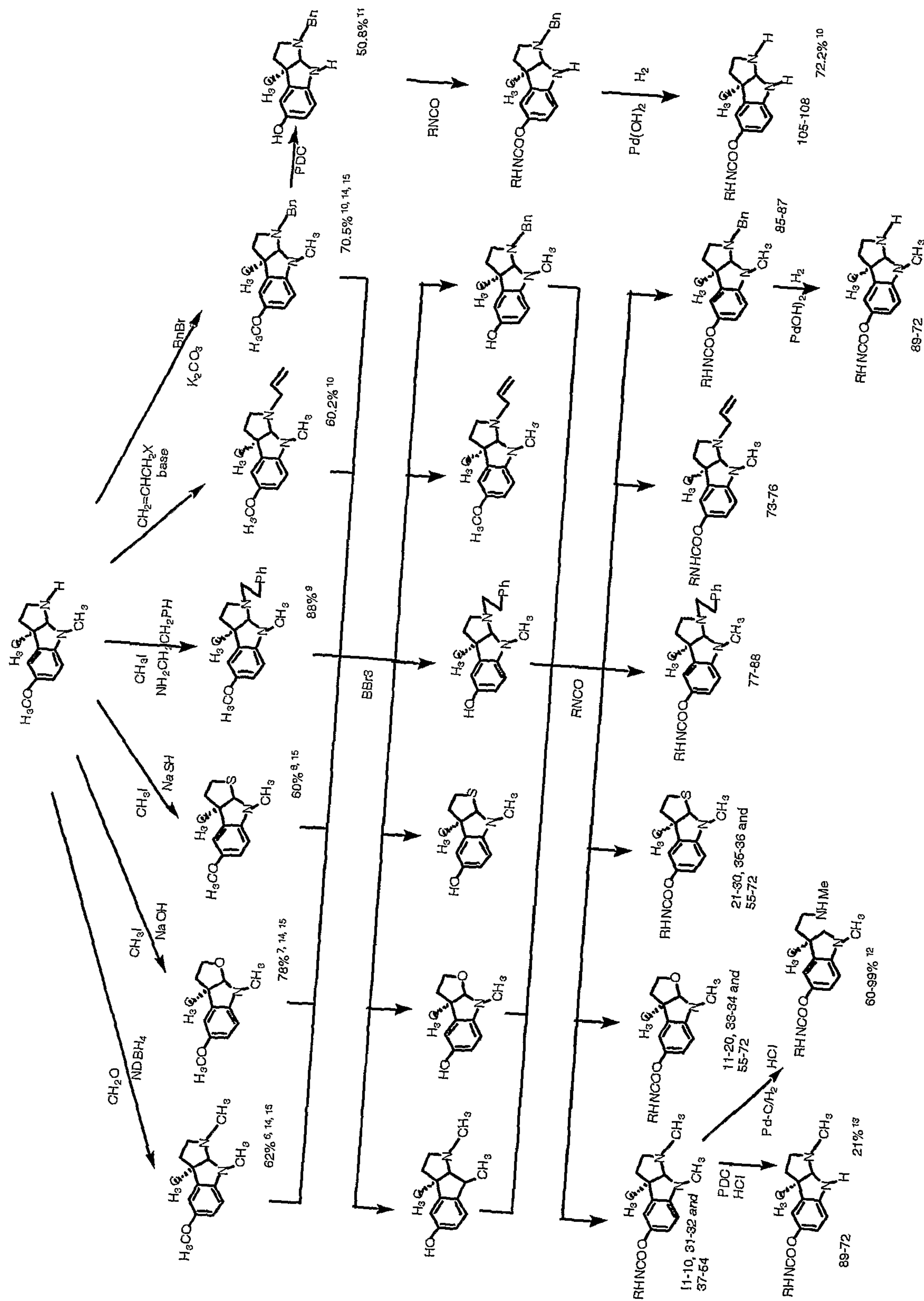
Figure 2. Transformation of (+)-N1-nor-esermethole to analogues of (+)-physostigmine
