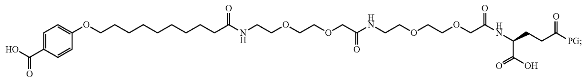
Chem. 80:
