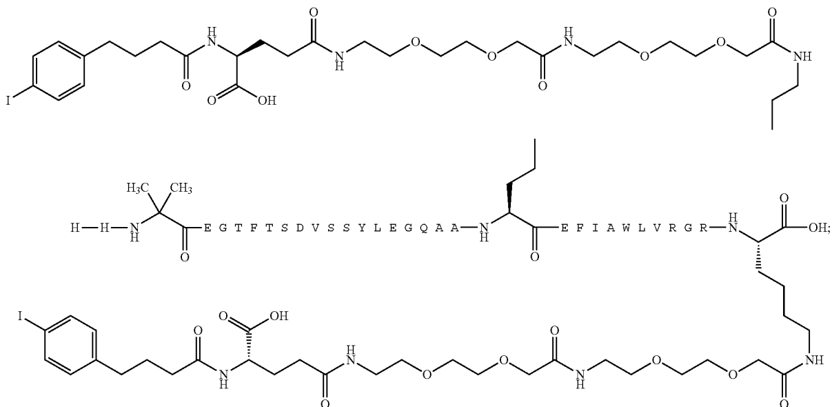
Chem. 31:
