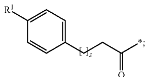
Chem. 3a:
