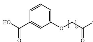
Chem. 2b:
