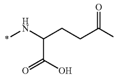
Chem. 7:
