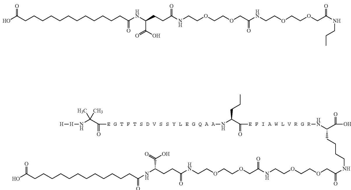
Chem. 23:
