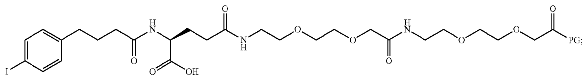
Chem. 72:
