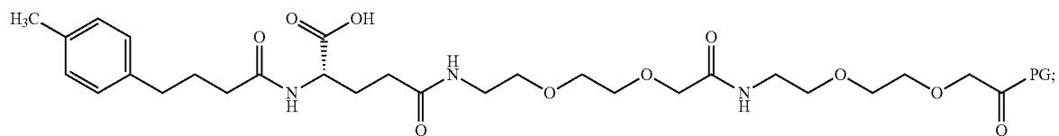
Chem. 76:
