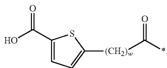
Chem. 4a:
