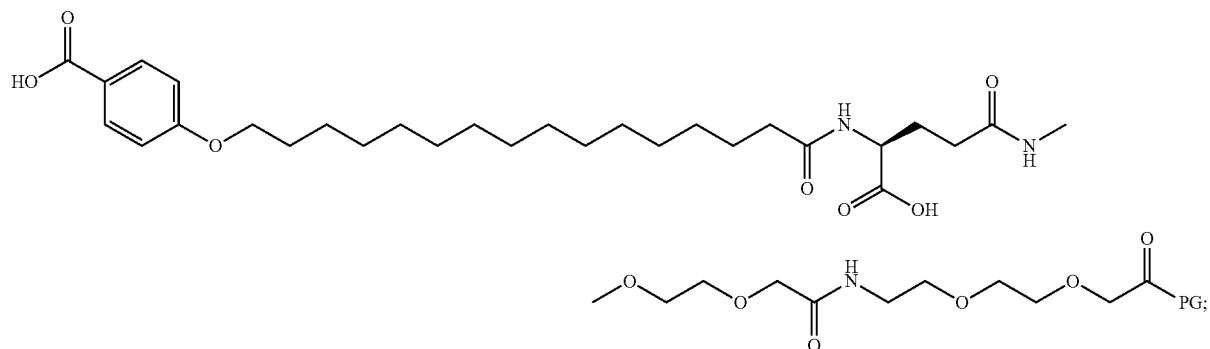
Chem. 73:
