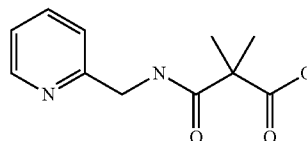
Chem. 19:
