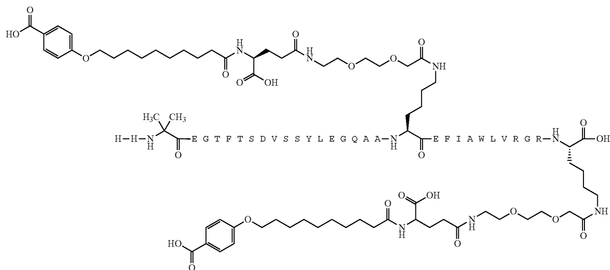
Chem. 34:
