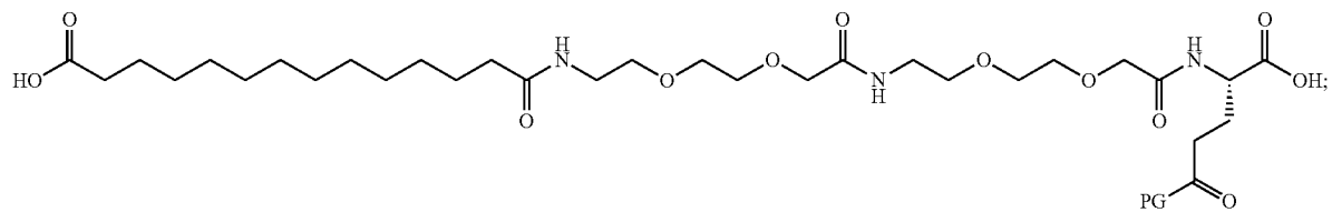
Chem. 78:
