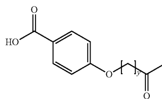
Chem. 2b:
