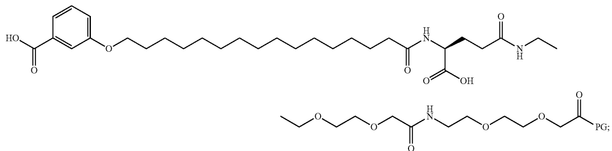
Chem. 78:
