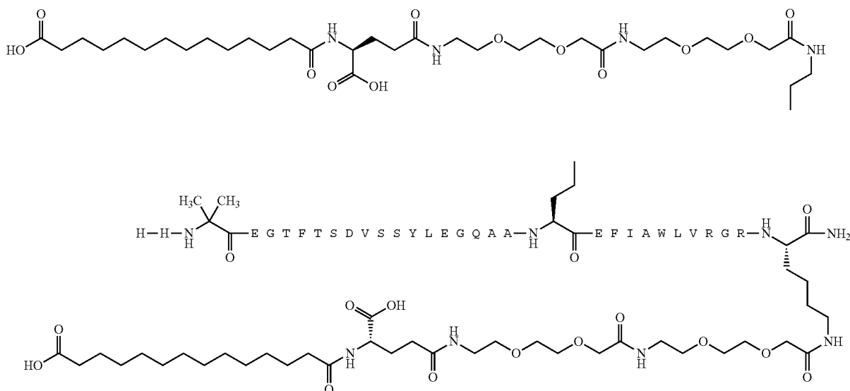
Chem. 26:
