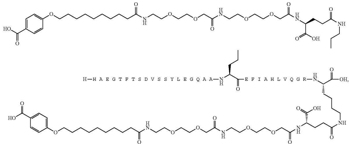
Chem. 55:
