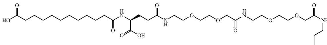
Chem. 27:
