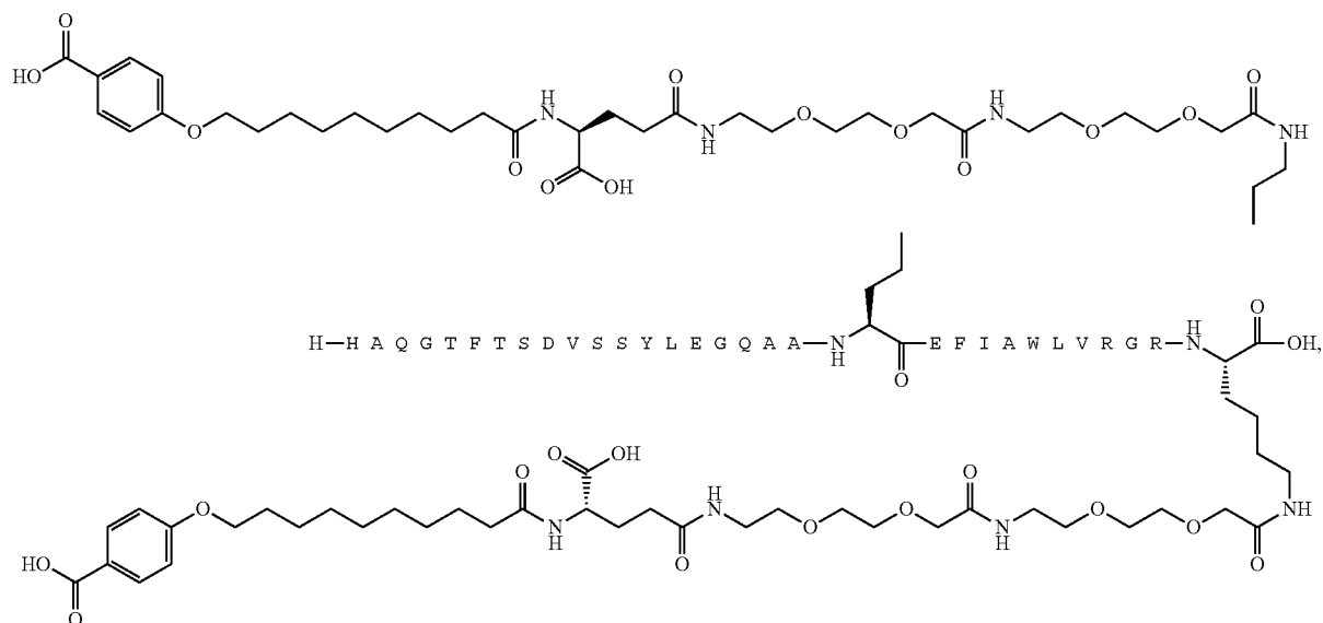
Chem. 56:
