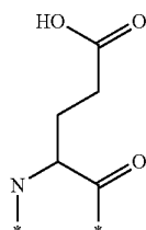
Chem. 7:
