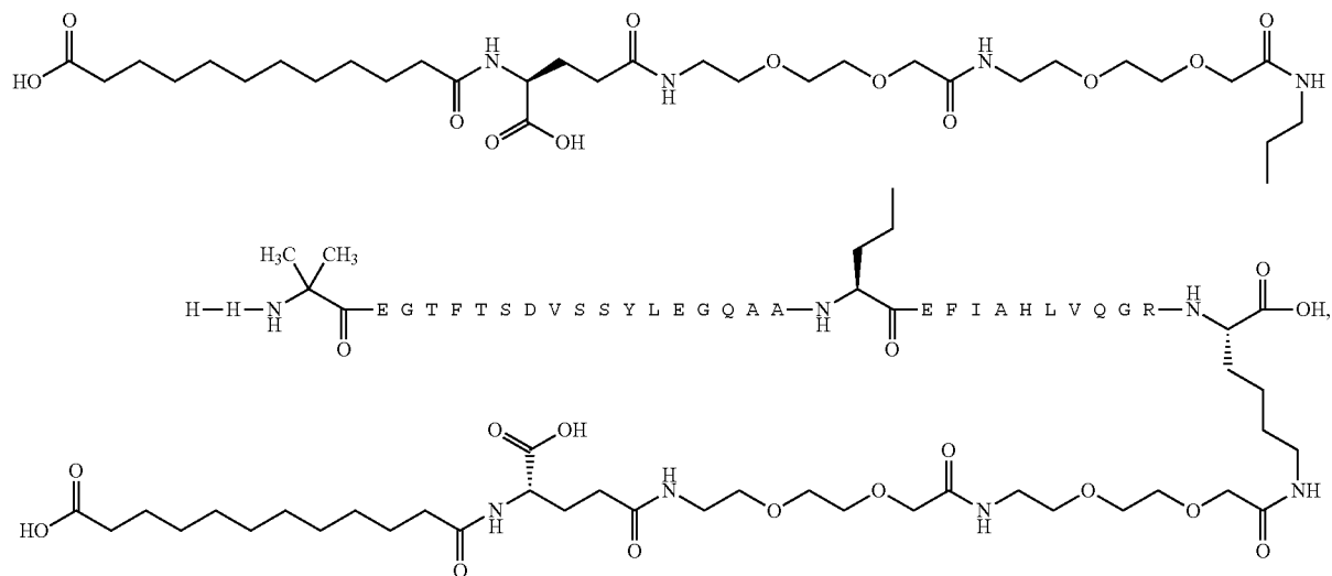
Chem. 40:
