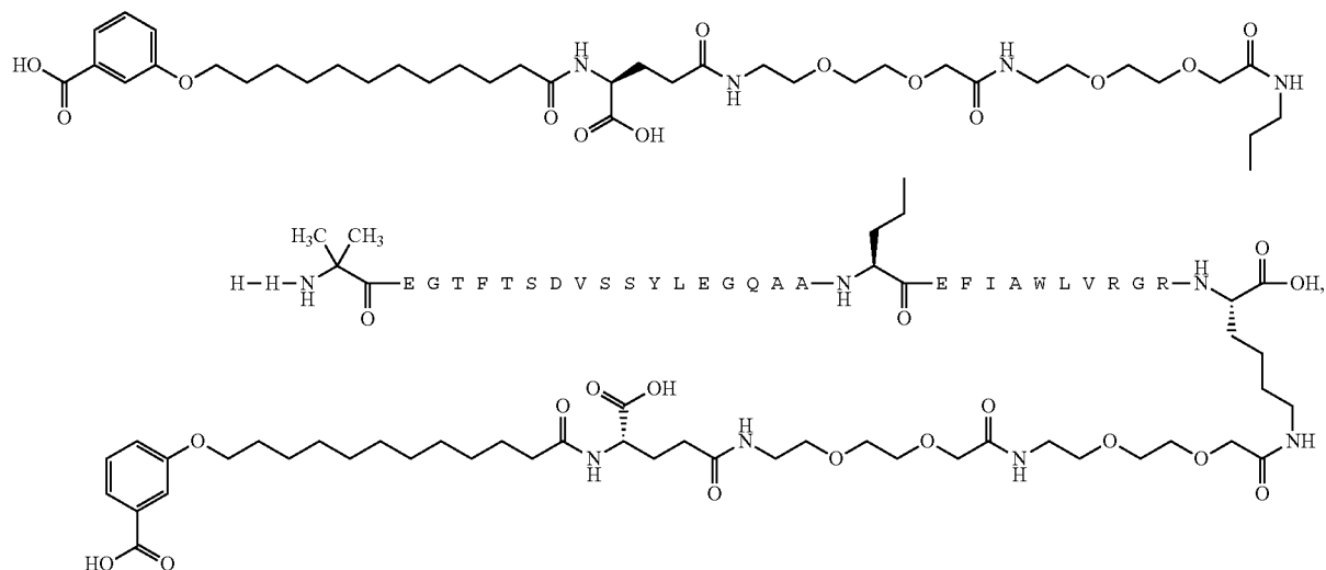
Chem. 35:
