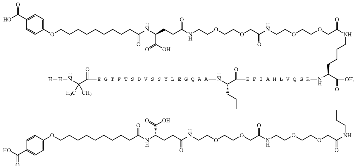
Chem. 36:
