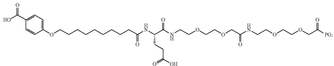
Chem. 82:
