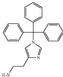
Chem. 13:
