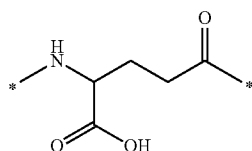
Chem. 7:
