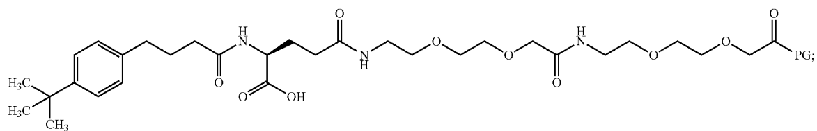
Chem. 80:
