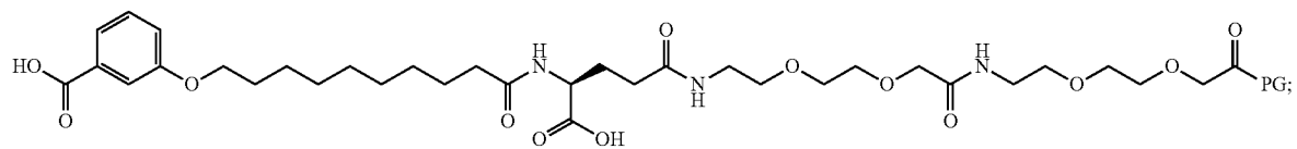
Chem. 76:
