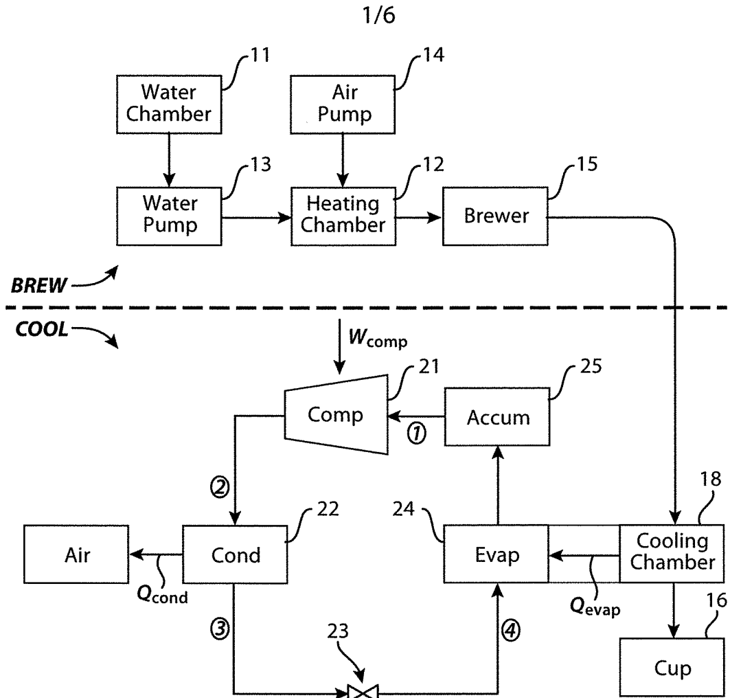
Schematic layout and Heat Flow diagram
