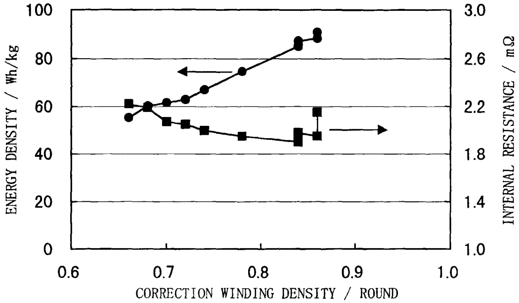
FIG. 4 (a) ONE SIDE THICKNESS OF POSITIVE ACTIVE MATERIAL LAYER : WITH 100 μ m
