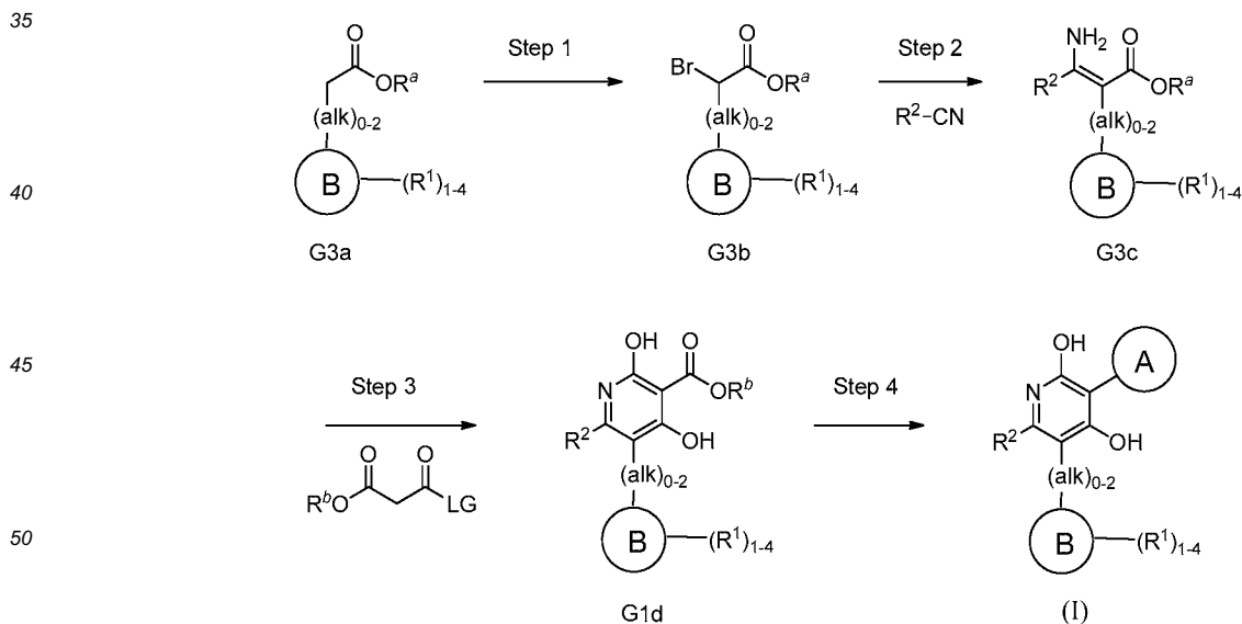
Scheme 3
