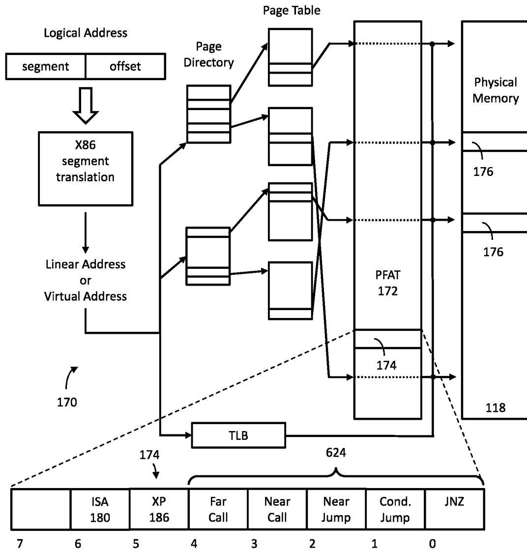
Fig. 1d – Memory Mapping
