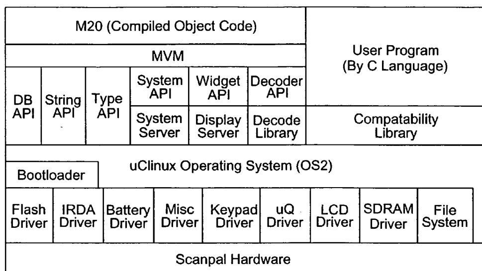
Software Block Diagram
