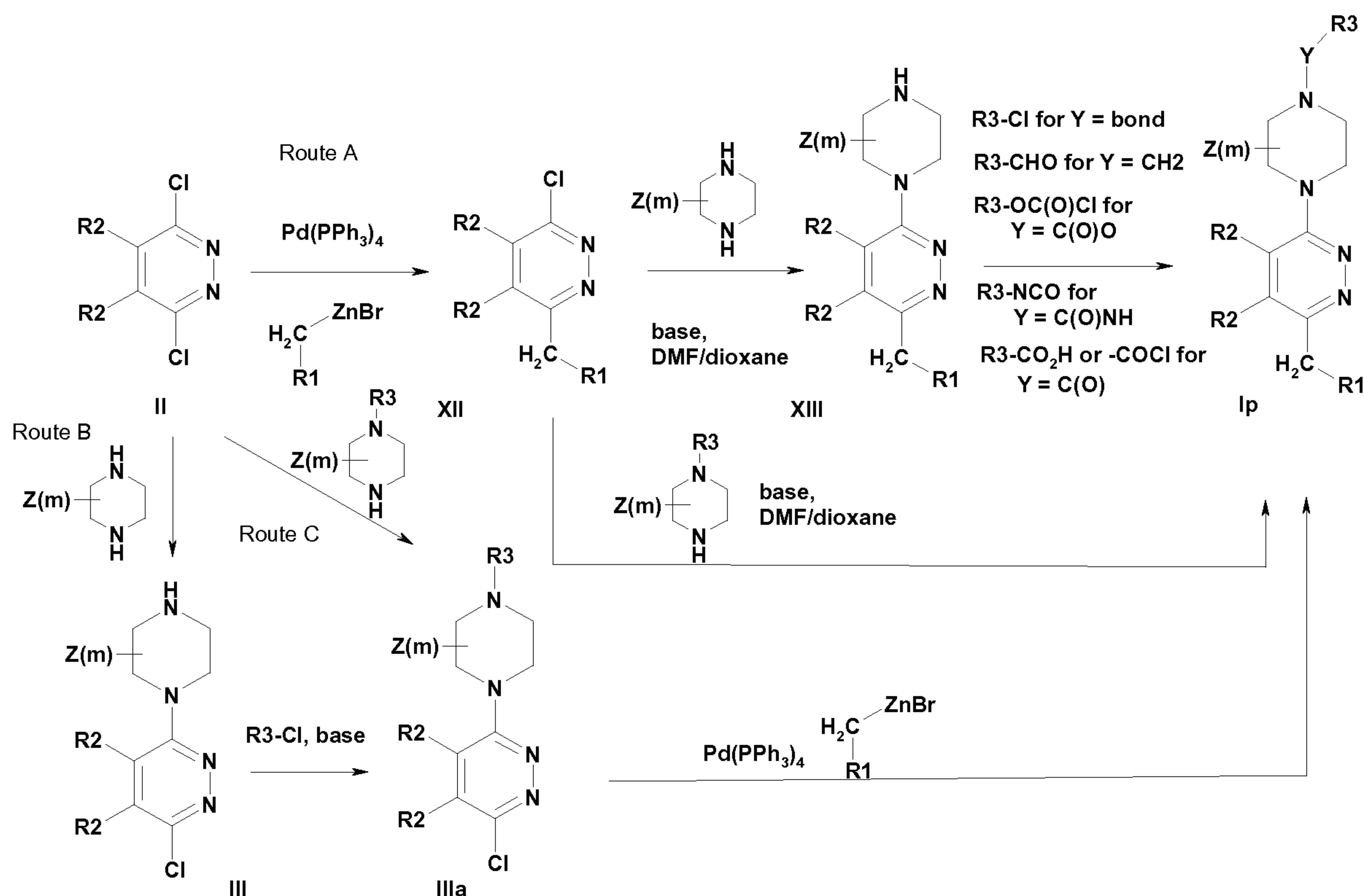
SCHEME 6
