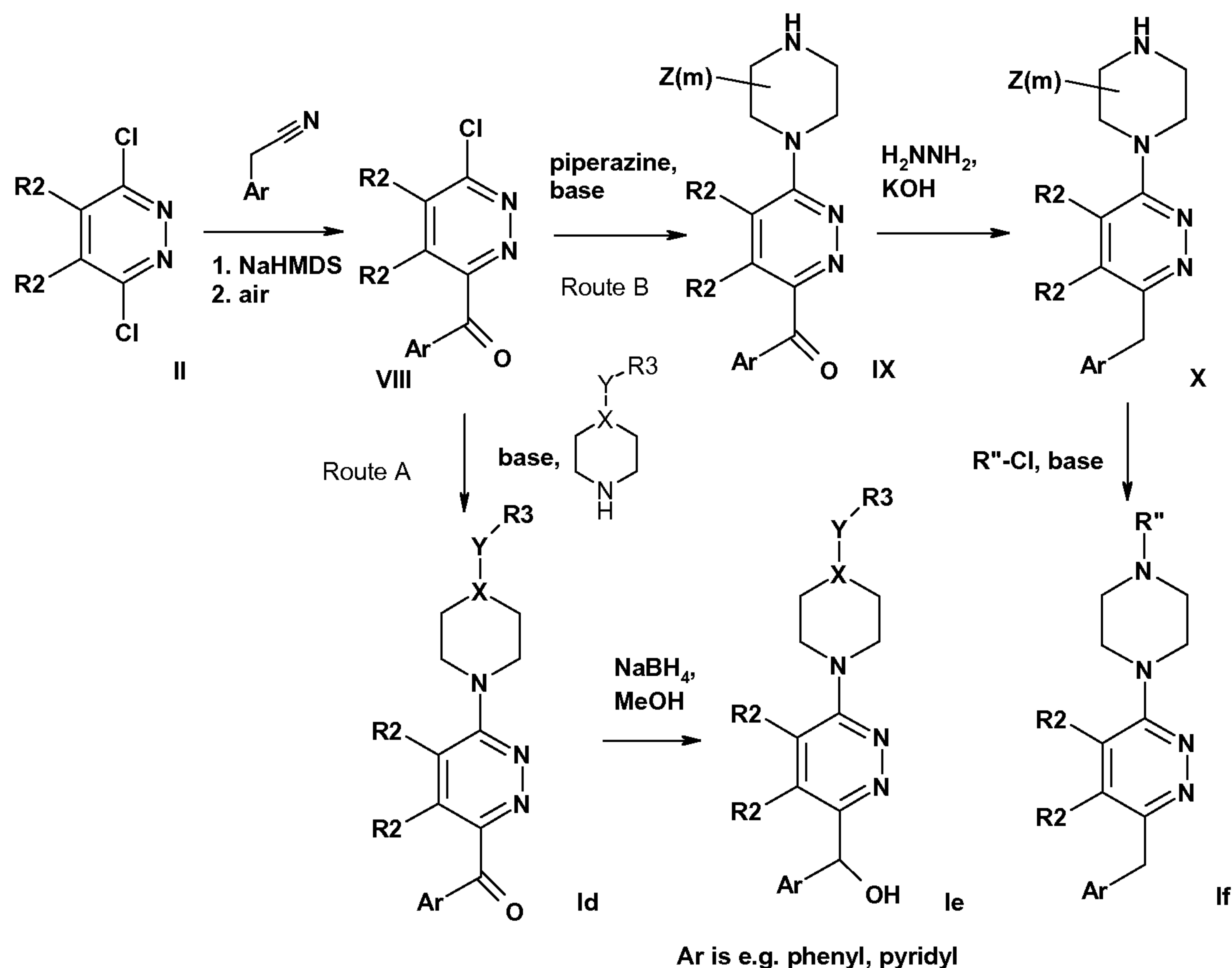
SCHEME 4
