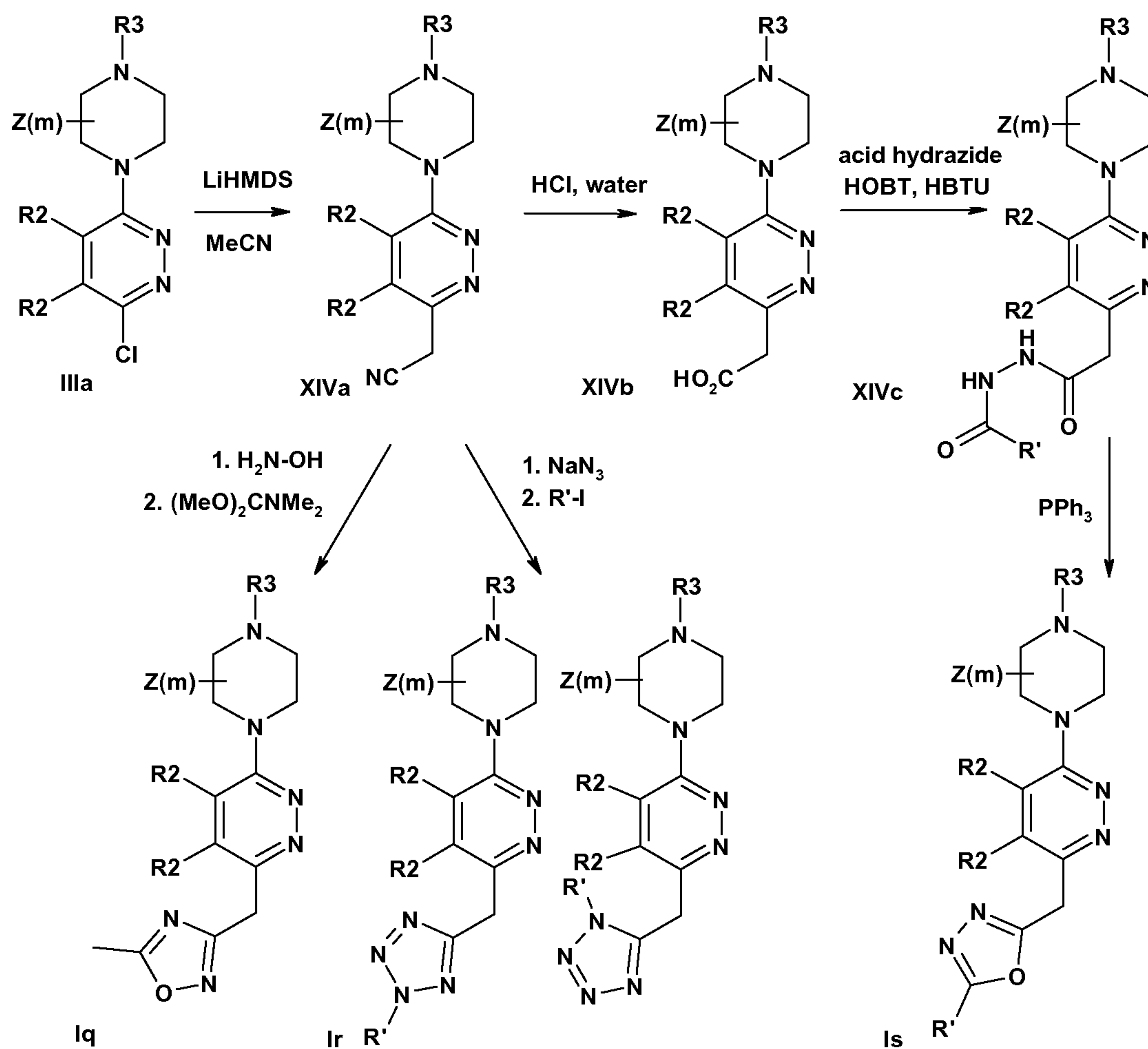
SCHEME 7
