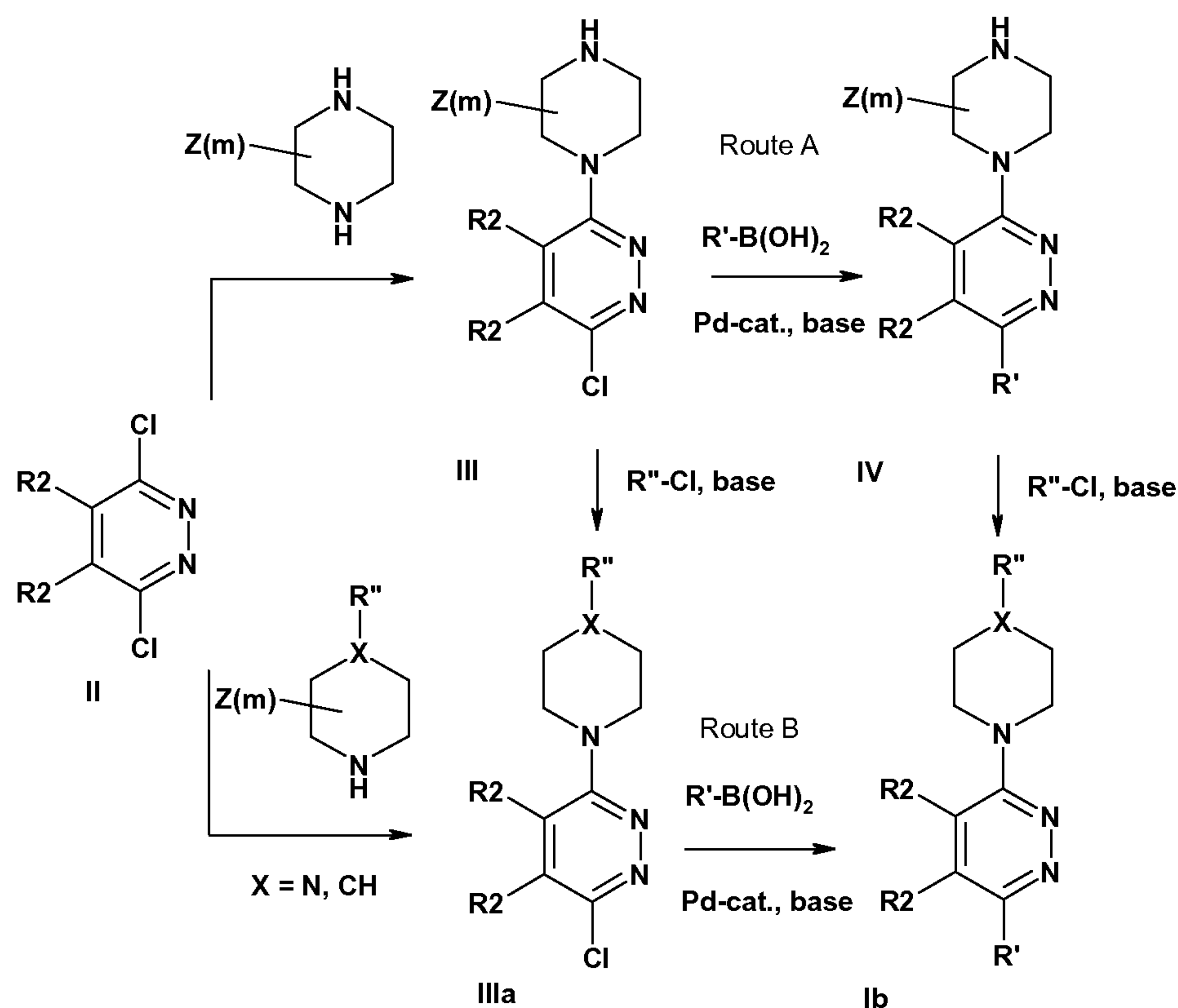
SCHEME 2
