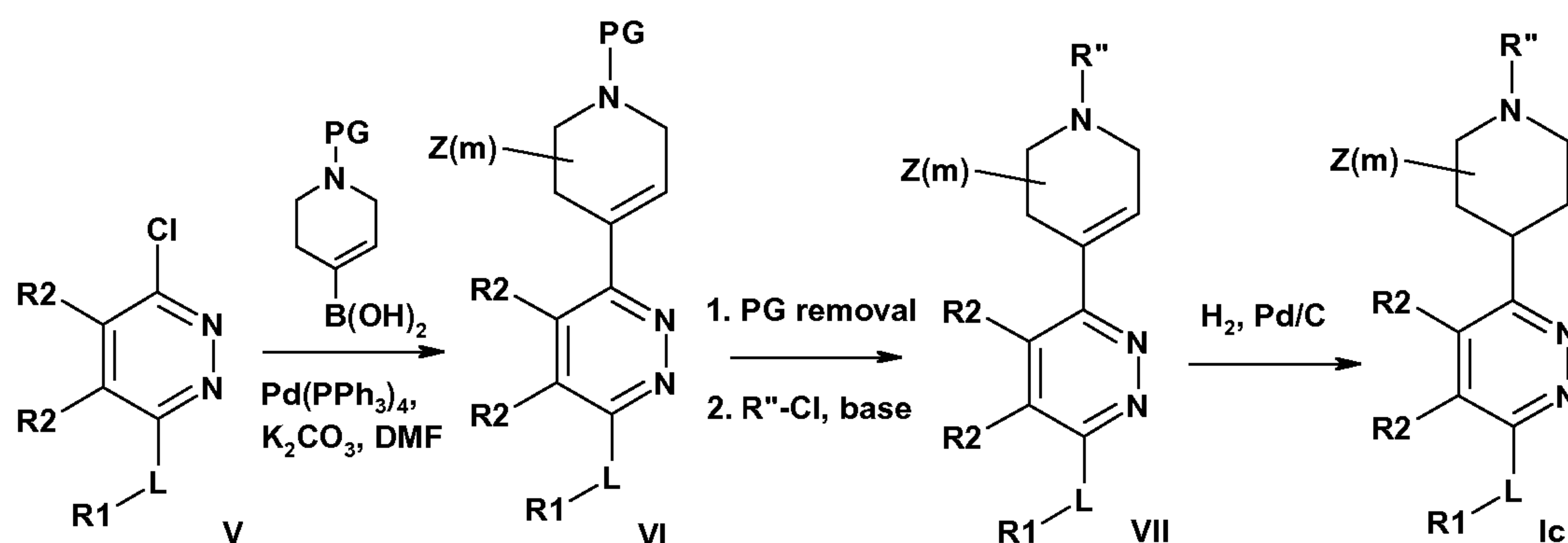
SCHEME 3
