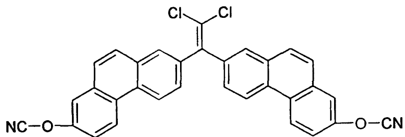
17 phenanthrol
