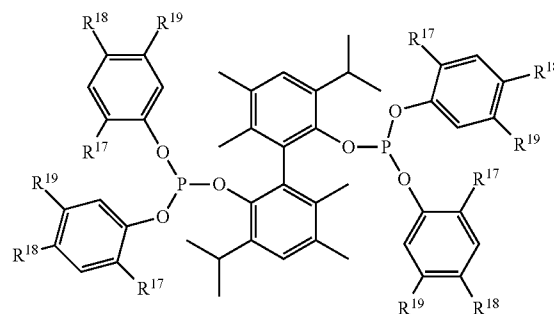
Formula (IVa)
