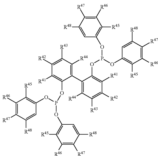
Formula XI
