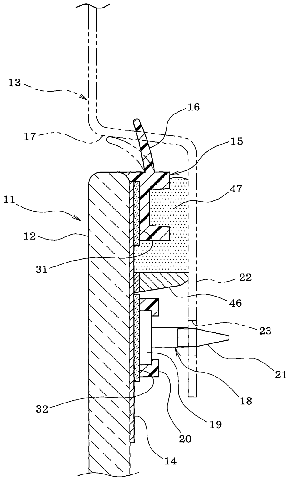
SECTIONAL VIEW TAKEN ALONG LINE B-B
