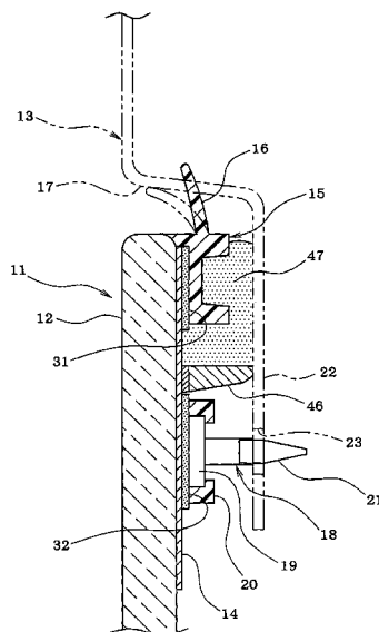
SECTIONAL VIEW TAKEN ALONG LINE B-B
