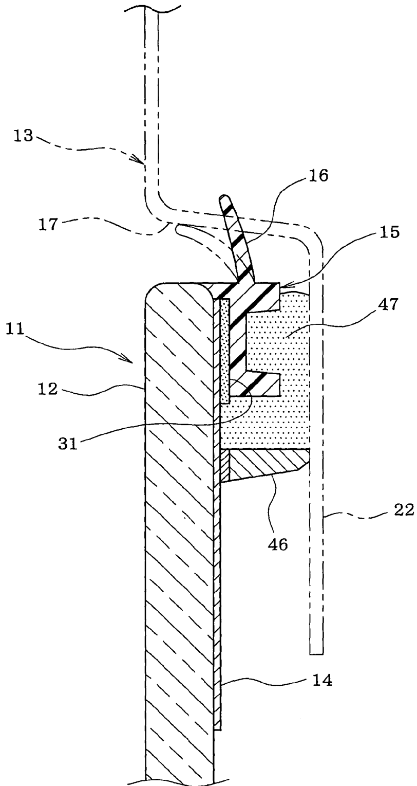
SECTIONAL VIEW TAKEN ALONG LINE A-A
