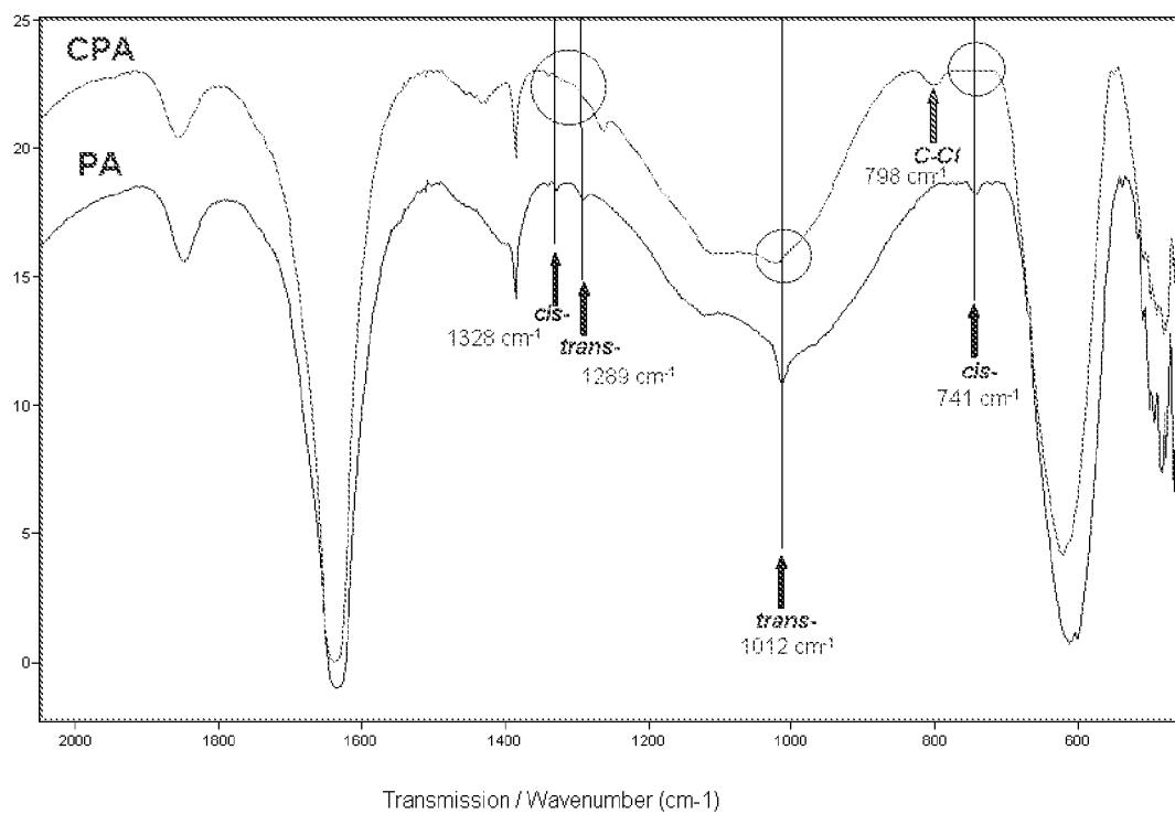
Figure 5. – FTIR for example gas phase produced CPA
