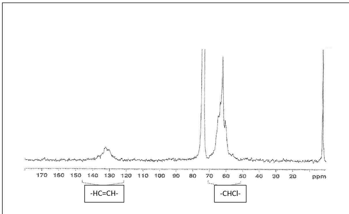
Figure 2 – ^{13}\text{C} NMR for CPVC
