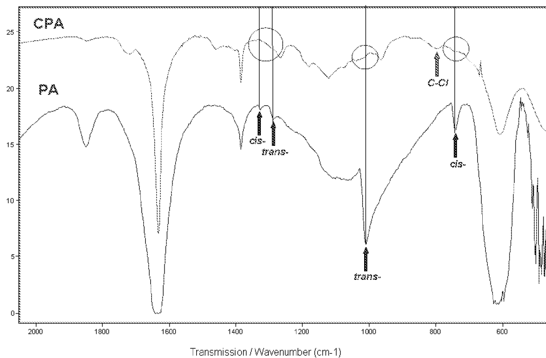
Figure 4. - FTIR for comparative example slurry produced CPA
