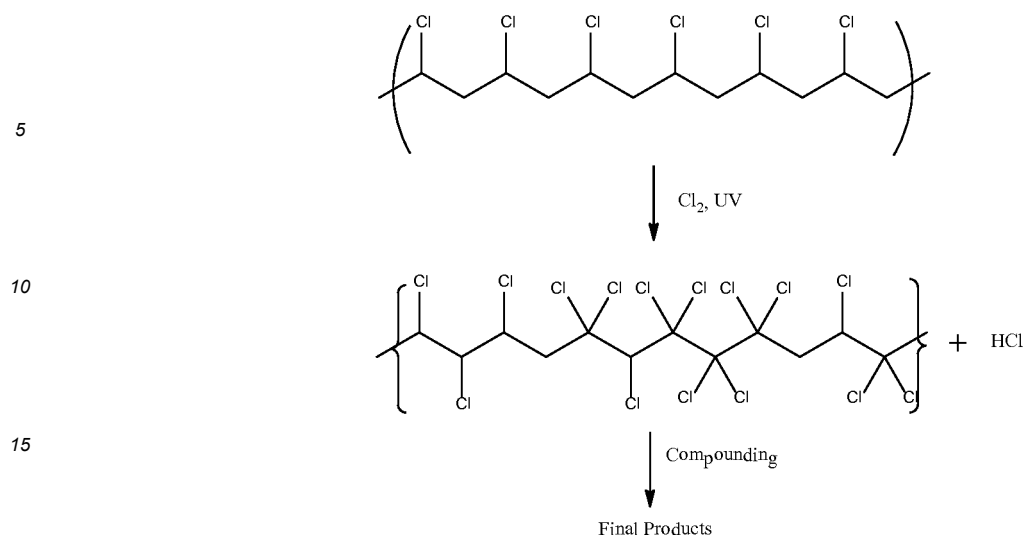
Graphic 1. Current CPVC technology: slurry process in water
