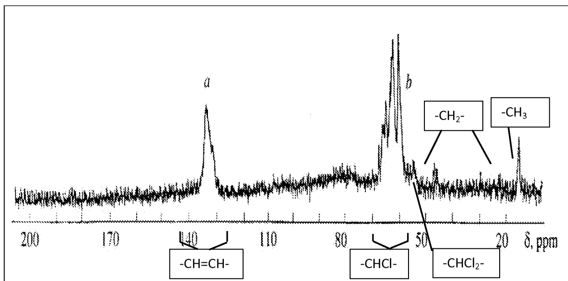
Figure 3 - ^{13}\text{C} NMR for CPA made by slurry process in DMF
