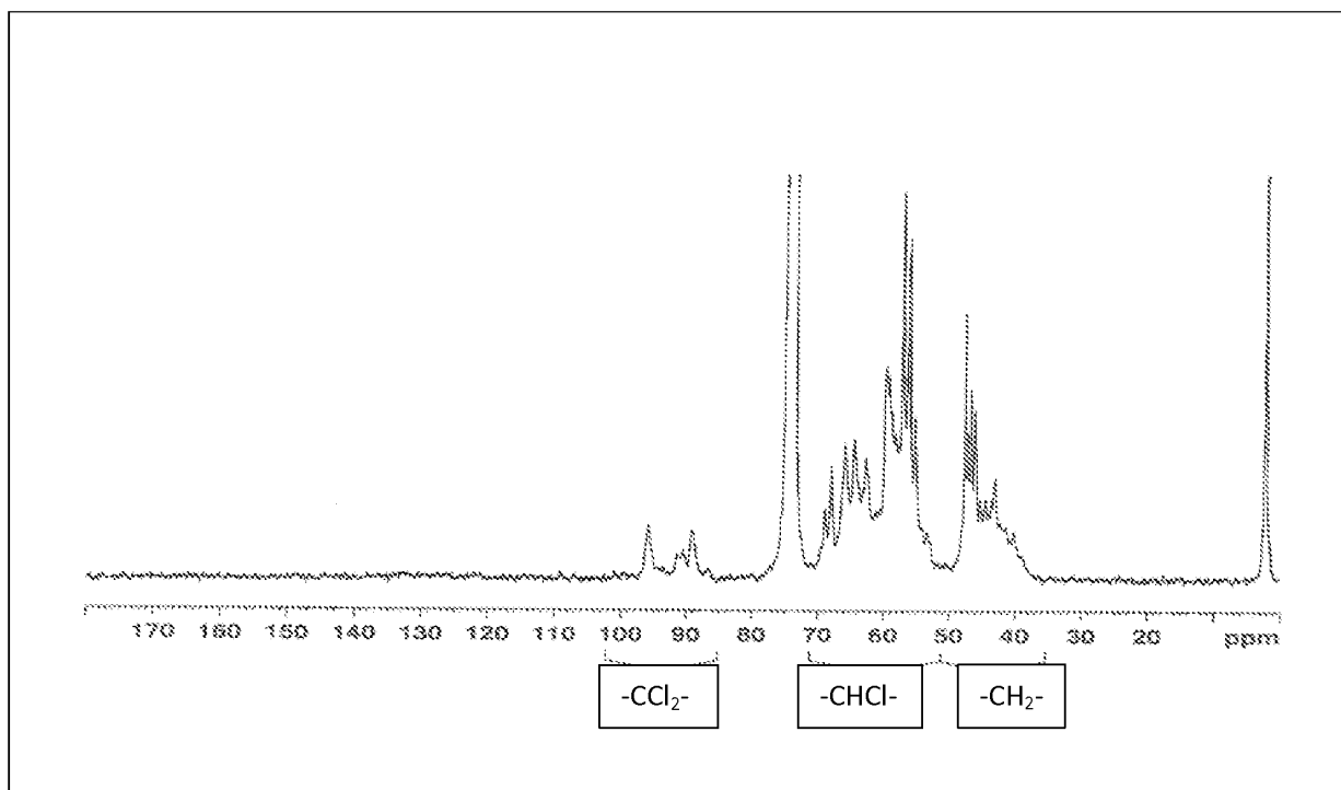
Figure 2 – ^{13}\text{C} NMR for CPVC
