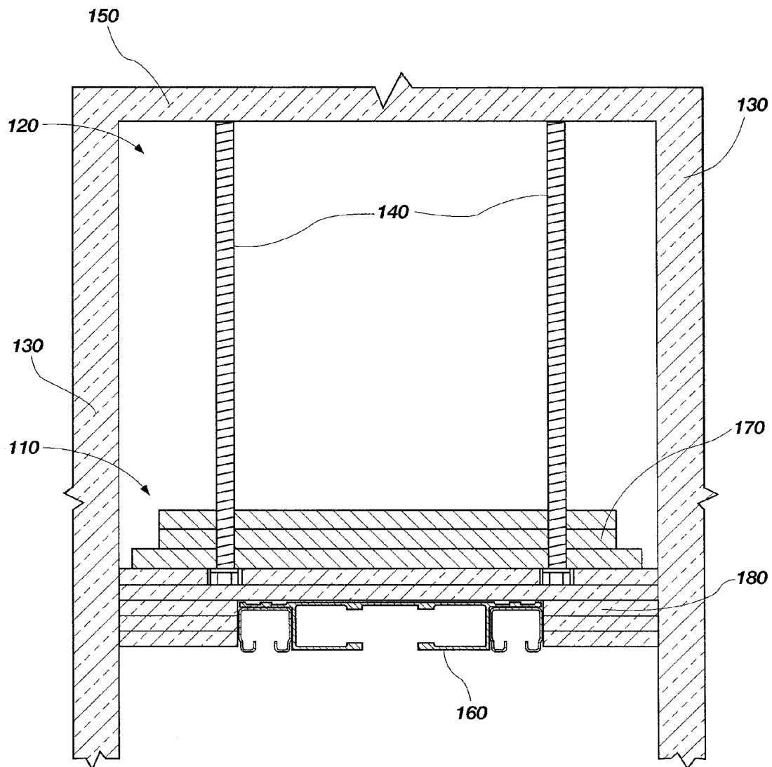
FIG. 1 (PRIOR ART)
