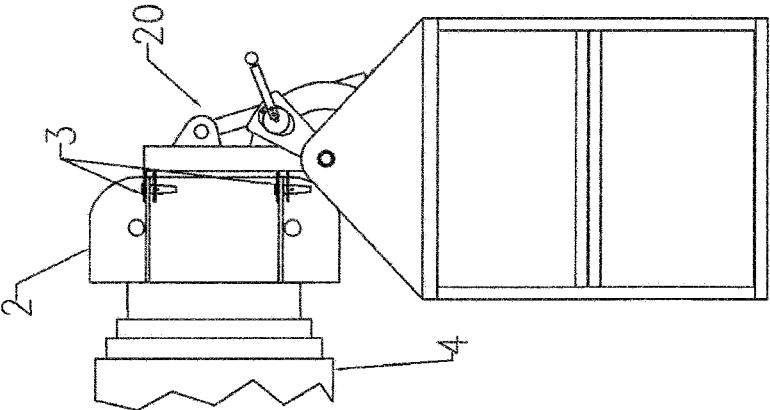
FIG. 5 PRIOR ART
