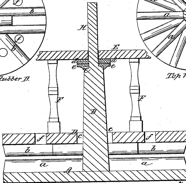
Vertical Section.
