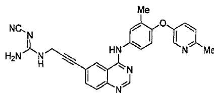
N-cyano-N'-(3-{4-[3-Methyl-4-(6-methyl-pyridin-3-yloxy)-phenylamino]-quinazolin-6-yl}-prop-2-ynyl)guanidine
