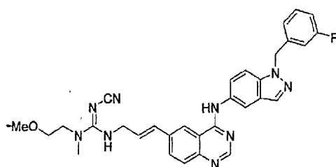
N-cyano-N'-(3-{4-[1-(3-Fluoro-benzyl)-1H-indazol-5-ylamino]-quinazolin-6-yl}-allyl)-N''-(2-methoxy-ethyl)-N'''-methylguanidine
