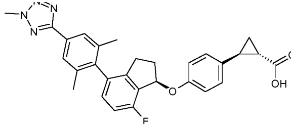
Example 45 in WO 2013/178575
