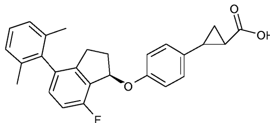
Example 33 in WO 2013/178575
