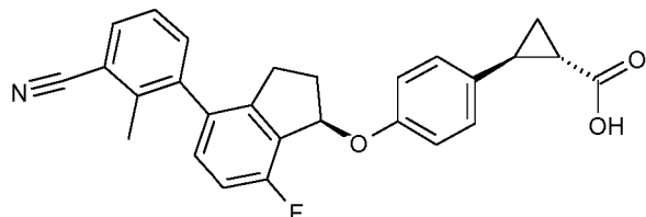
Example 54 in WO 2013/178575
