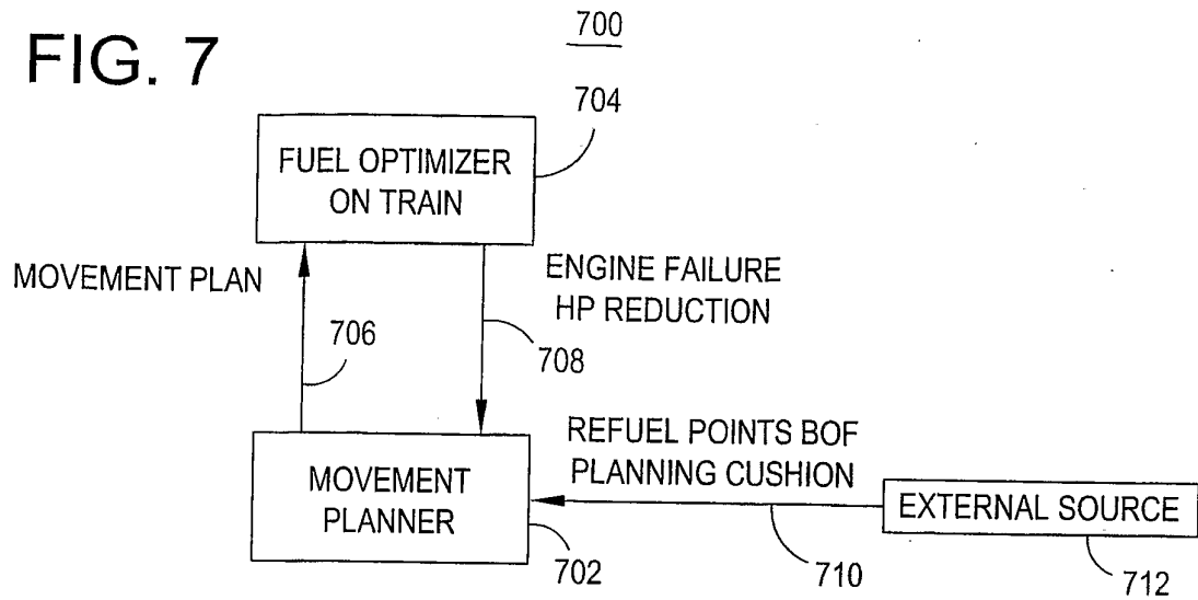
INTERFACE TRAIN LEVEL TO MOVEMENT PLANNER
