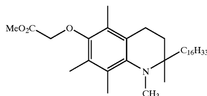
1-Aza-N-methyl- \alpha -tocopherol-6-yloxy-methyl Acetate (41)
