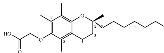
2,5,7,8-Tetramethyl-2(R-(heptyl)chroman-6-yloxy) acetic Acid (23)
