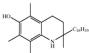
1-Aza- \alpha -tocopherol (38)
