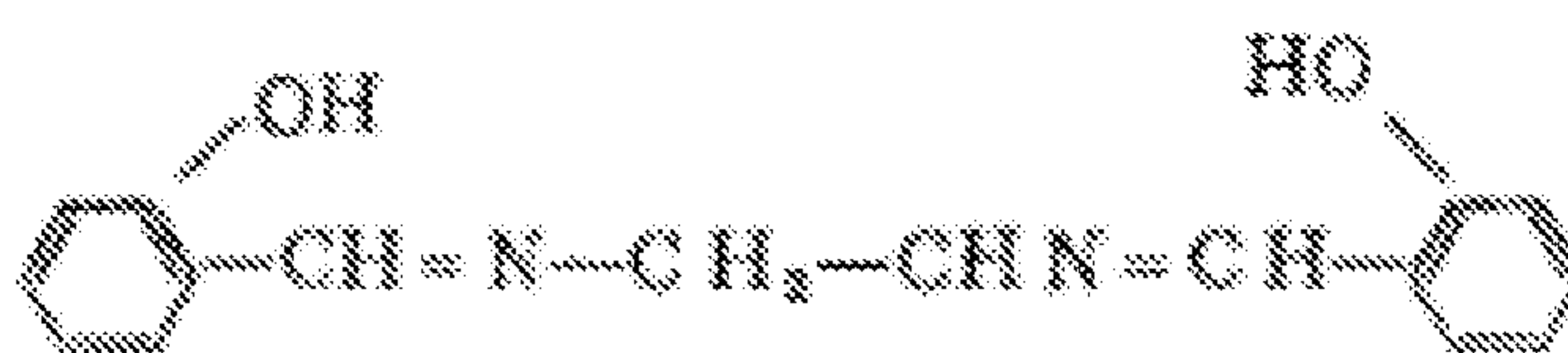
Formula VI - N,N'-bis(salicylidene) ethylenediamine
