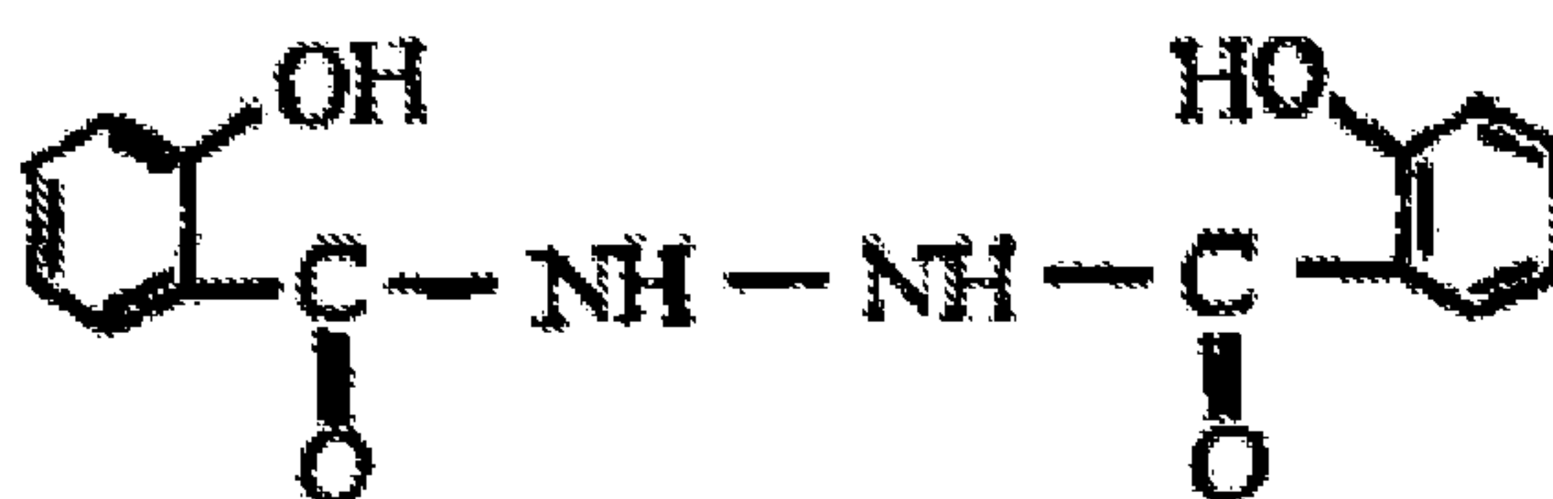
Formula III - N,N'-bis(salicyloyl)hydrazine
