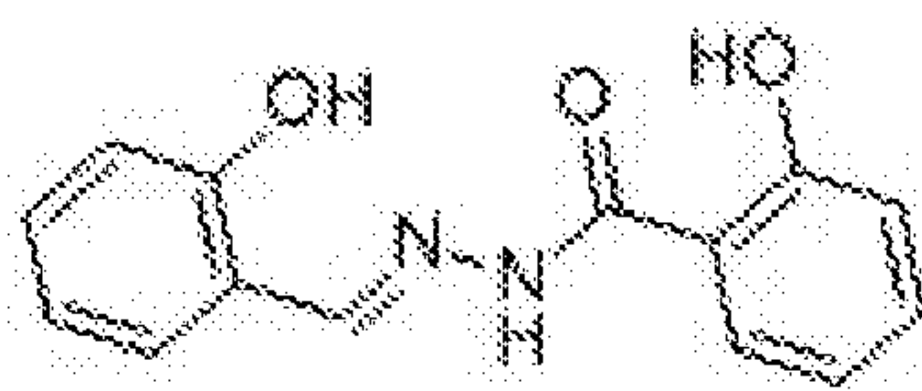
Formula I – N-salicylidene-N'salicyloyl hydrazide
