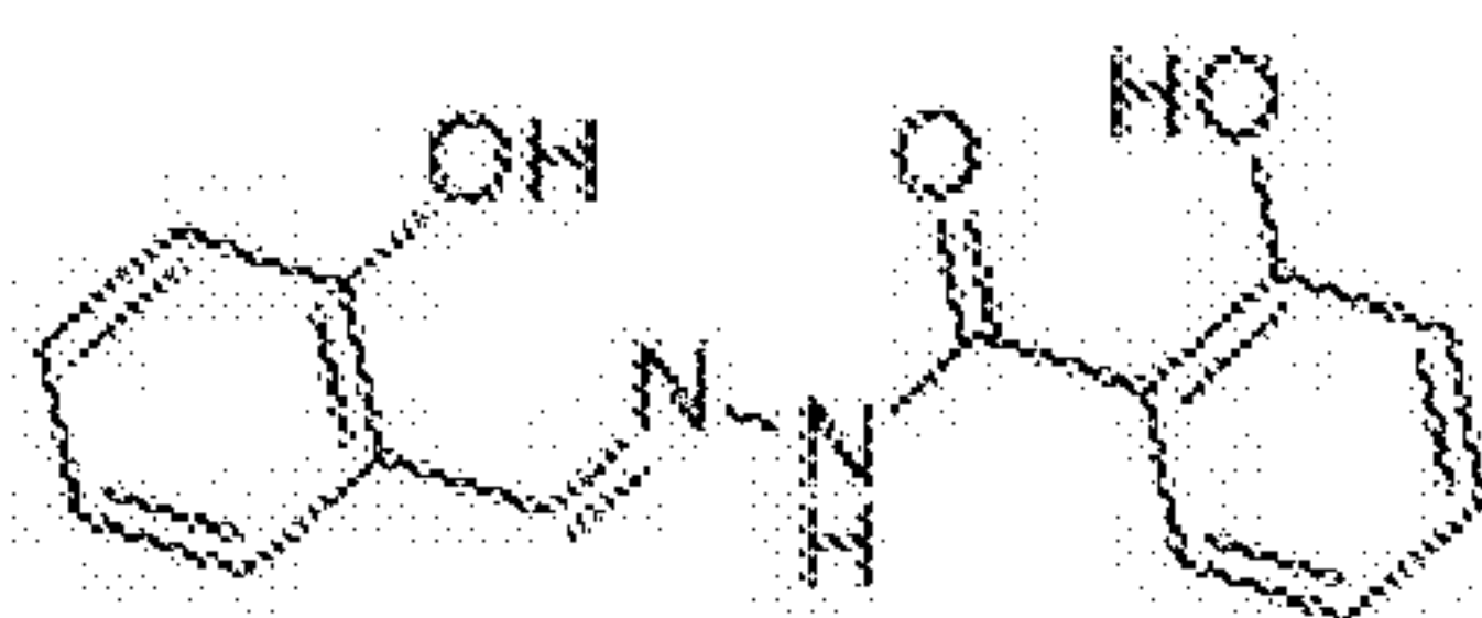
Formula I – N-salicylidene-N'salicyloyl hydrazide
