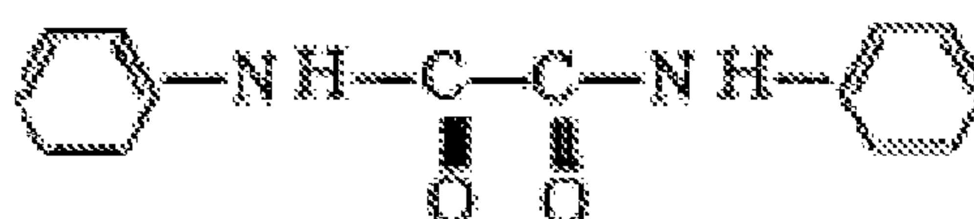
Formula VII – Oxanilide
