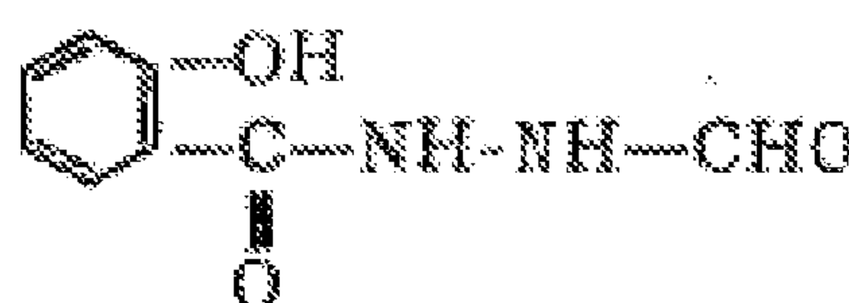
Formula IX - N-formyl-N'-salicyloyl hydrazine
