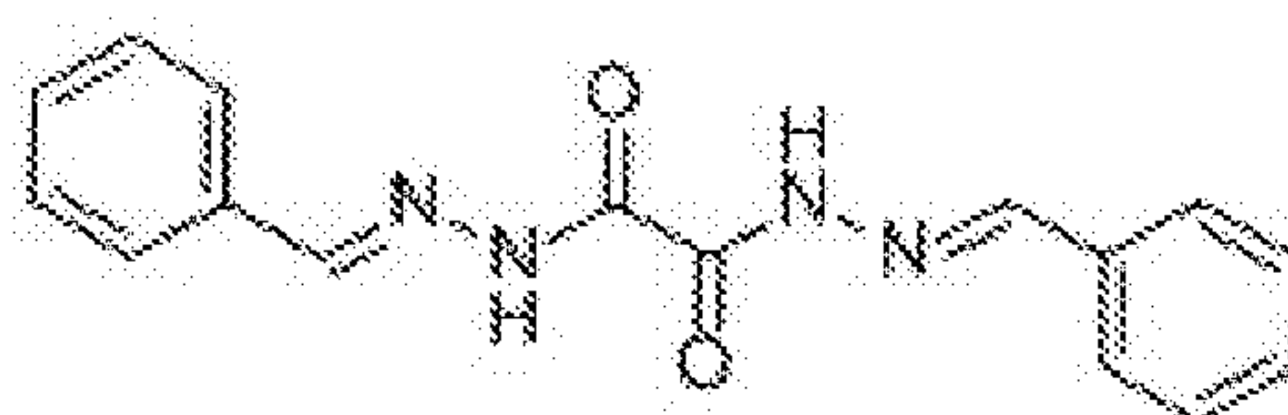
Formula II - oxalyl bis(benzylidenehydrazide)
