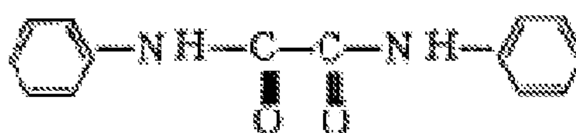
Formula VII – Oxanilide
