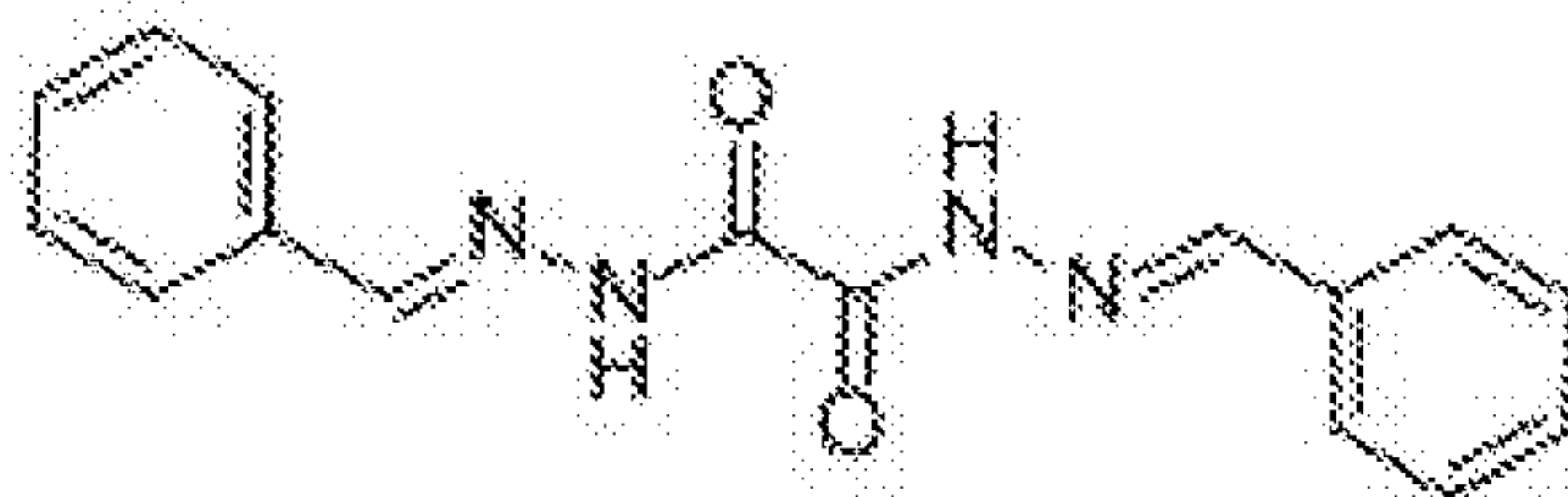
Formula II - oxalyl bis(benzylidenehydrazide)
