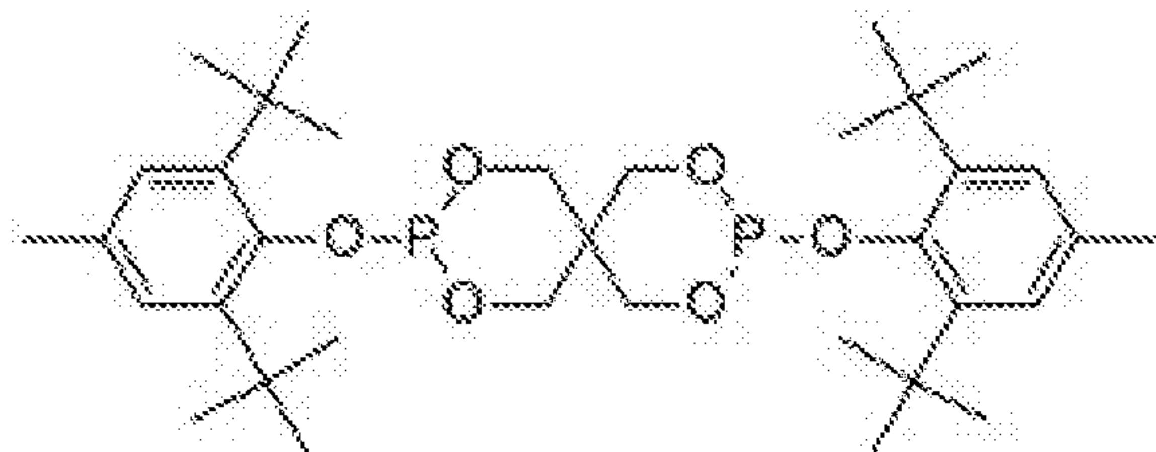
Formula XI - Bis(2,6-di-ter-butyl-4-methylphenyl)pentaerythritol-diphosphite
