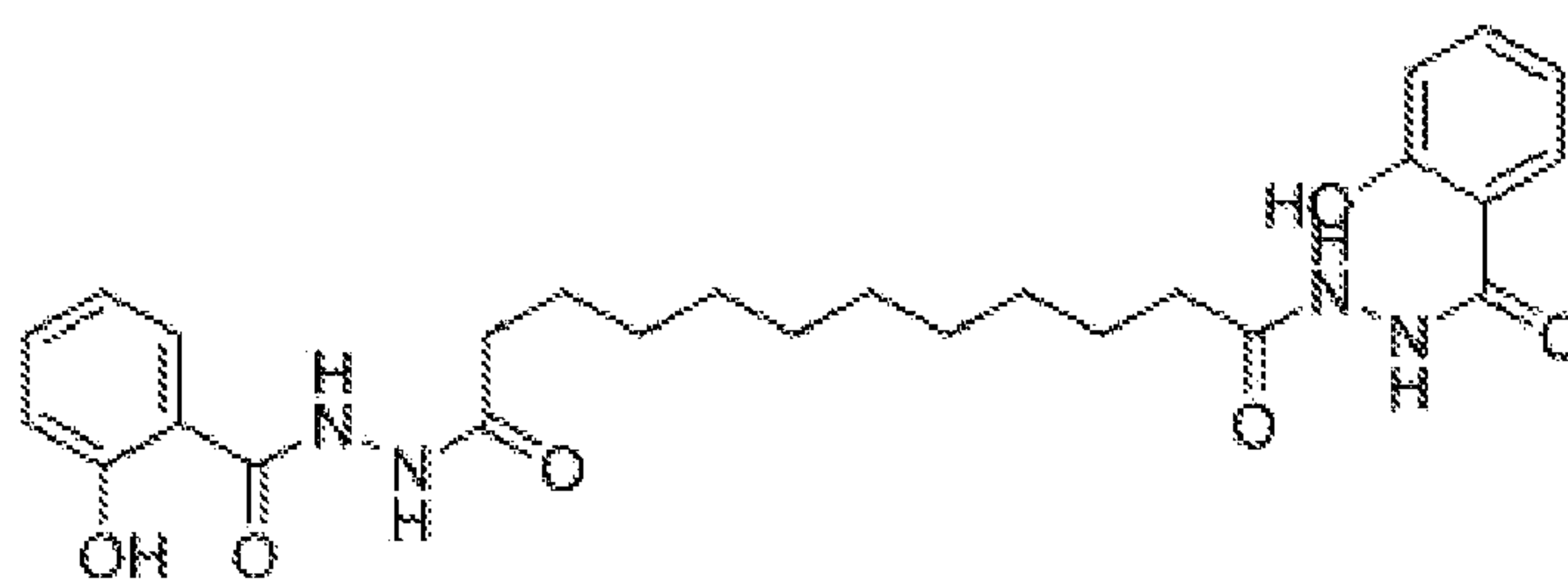
Formula X - Decamethylenedicarboxylic acid disalicyloylhydrazide
