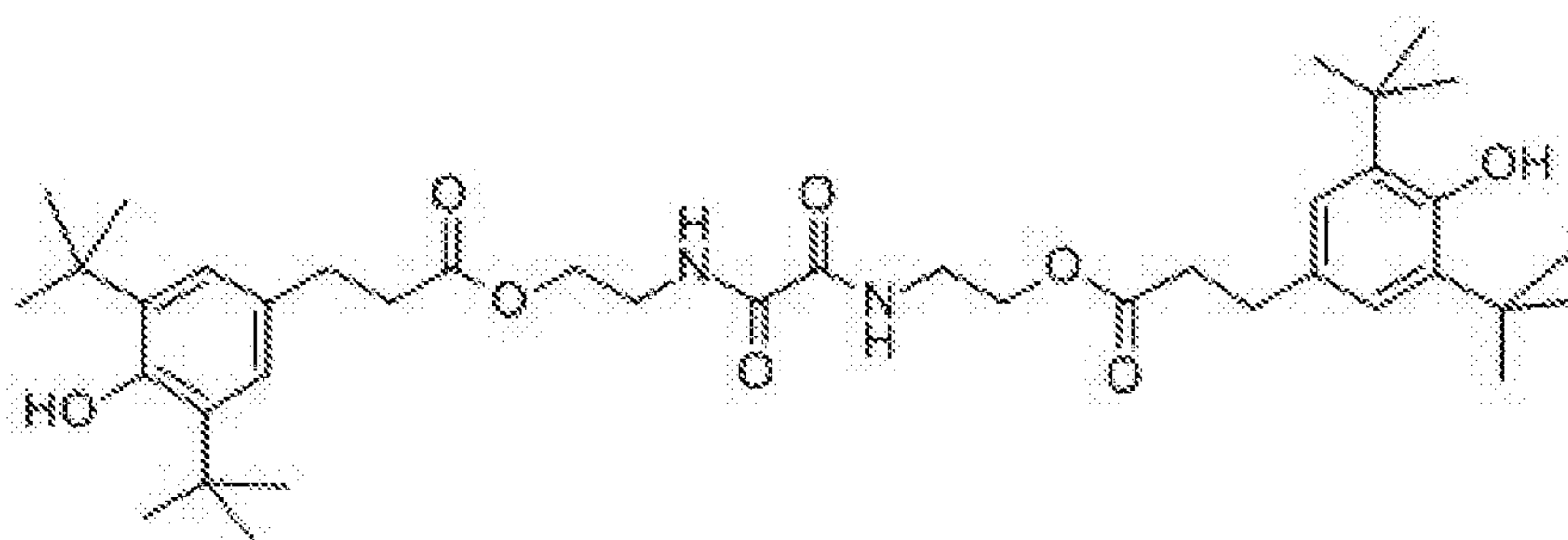
Formula V - 2,2'-oxamido bis[ethyl 3-(3,5-di-tert-butyl-4-hydroxyphenyl)propionate]
