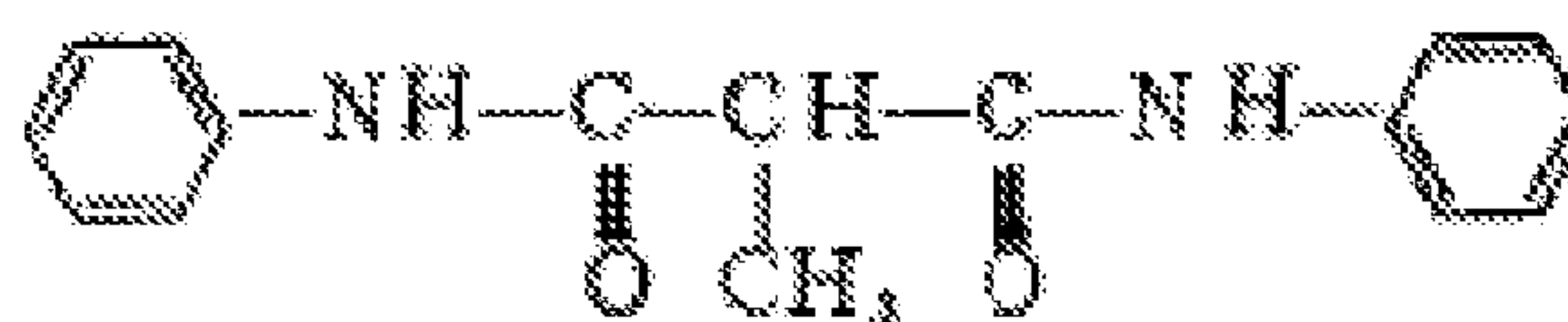
Formula VIII - Methylmalonic acid dianilide
