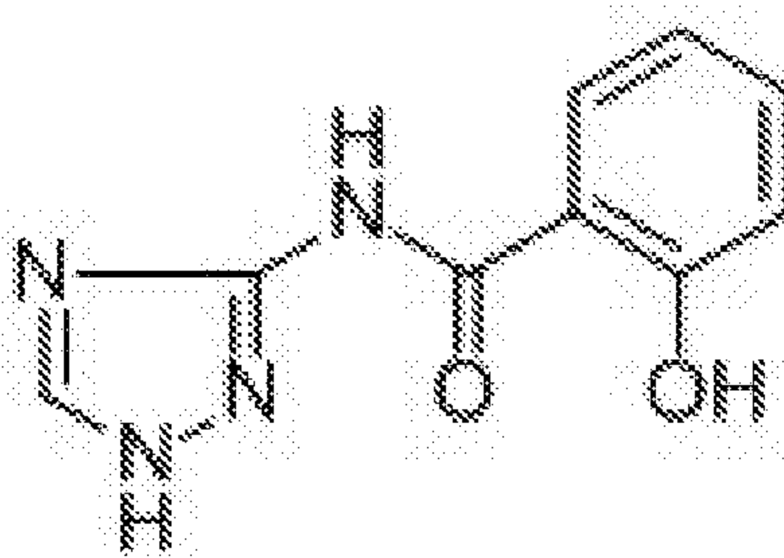
Formula IV - 3-(N-salicyloyl)amino-1,2,4-triazole
