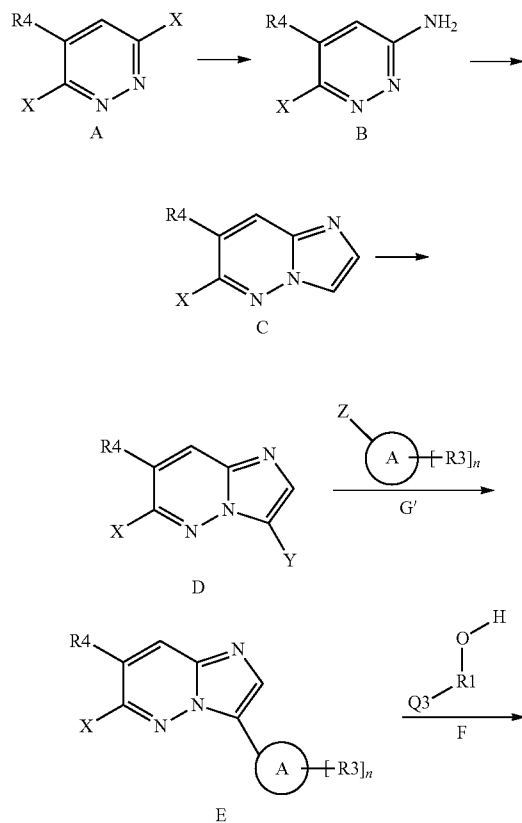
Scheme 3:
