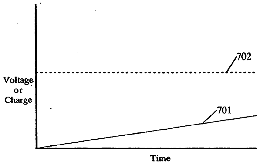
High Impedance Charge Profile
