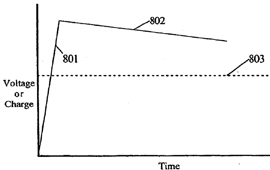
Low Impedance Charge Profile
